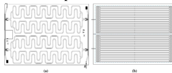
Fig.20. Roll-bond channel configuration used for a uncovered PVT and b covered PVT [100]
