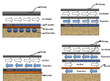
Fig.15. Classification of PV/T water collector based on water-flow pattern [64]
