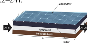
Fig-4. Layer diagram of PV/T air collector [136]
