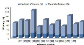
Fig.21. Summary of PVT water collector
