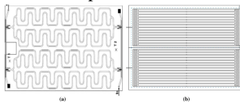
Fig.20. Roll-bond channel configuration used for an uncovered PVT and b covered PVT [100]
