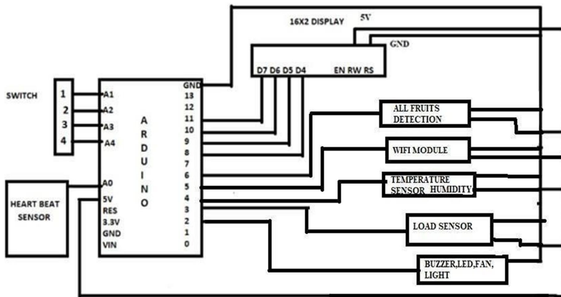
Block Diagram of fruits spoilage detection
