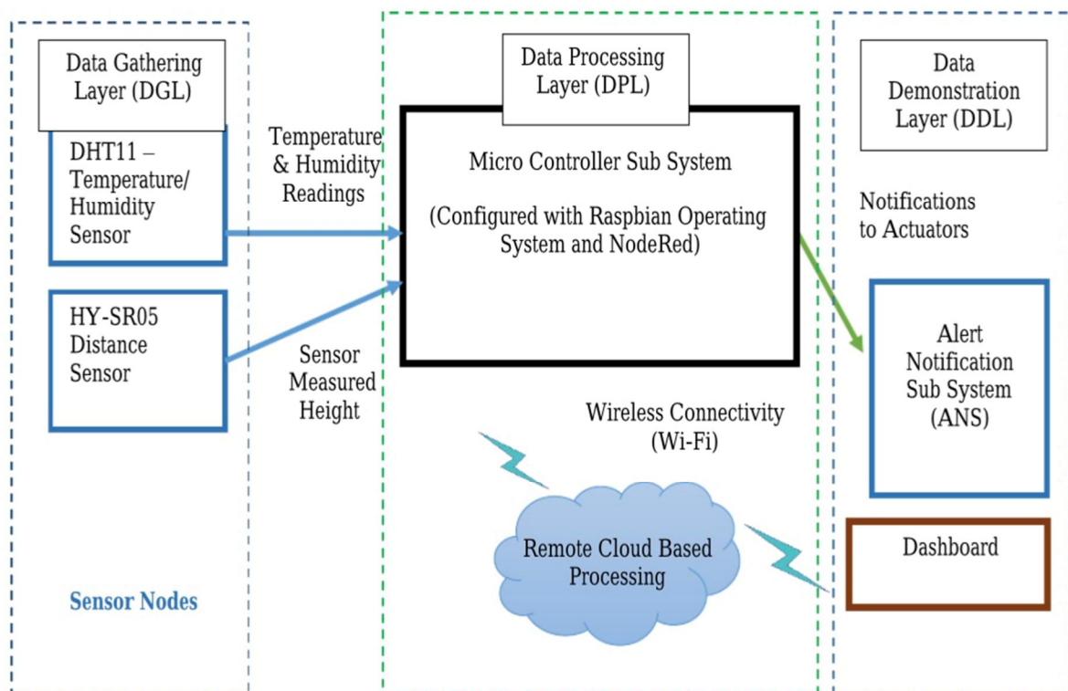
Fig. 1 System Overview of IOT based Smart Waste Bin Model
