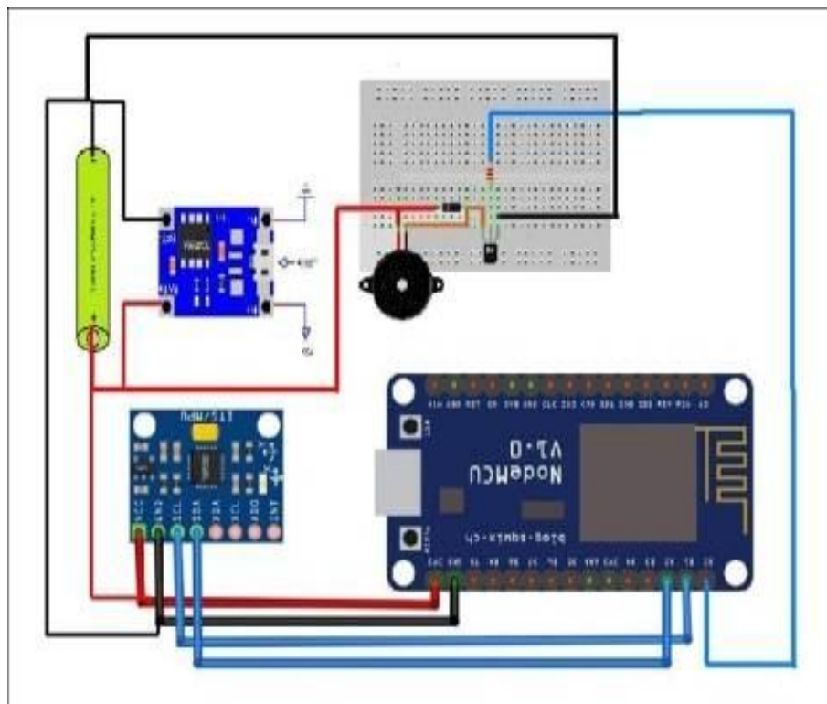
Fig.1 Circuit Diagram
