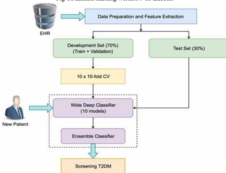
Fig 1:Machine learning workflow on diabetes
