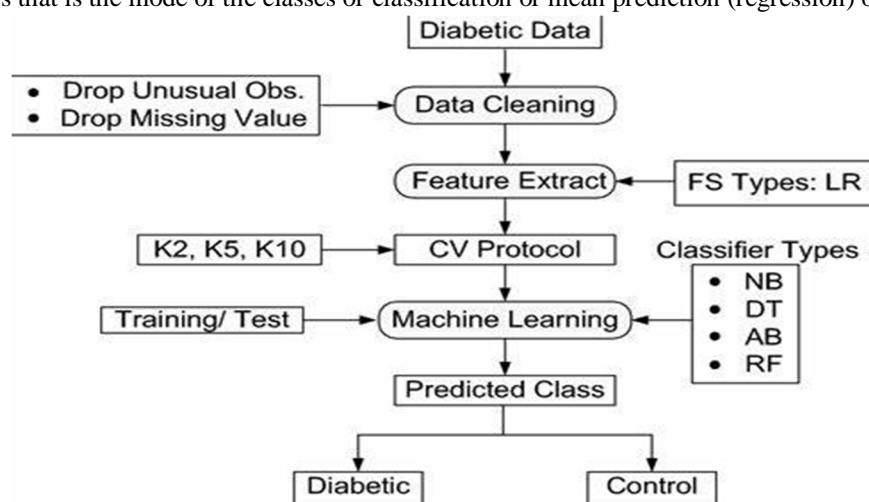
Fig 2: Classification of diabetes using machine learning
