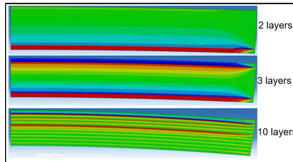
Figure 11. S_{11} (x dir.) Stress contours – elastic material properties.
