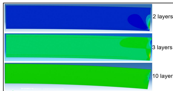
Figure 12. S_{22} (y dir.) Stress contours – elastic material properties
