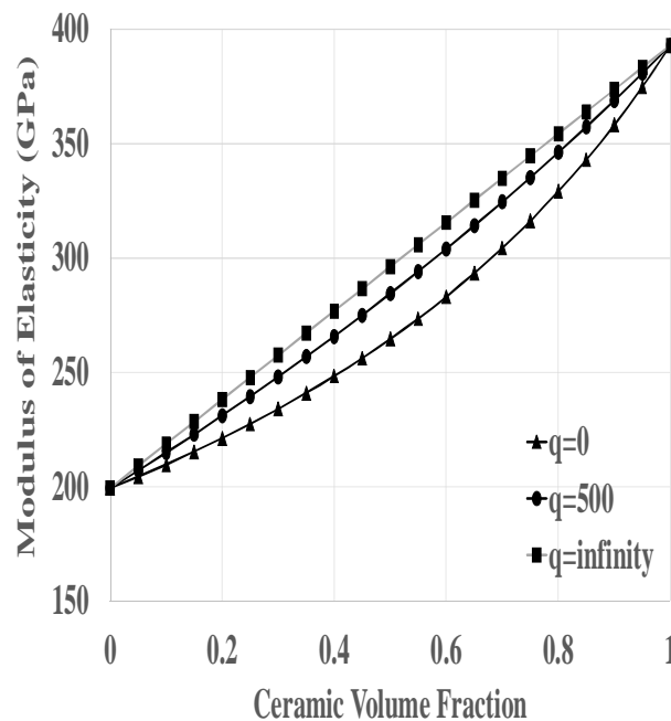
Figure 3. Predicted modulus of elasticity of nickel-alumina material using Equation 15 for q equaling 0, 500 and tending to infinity
