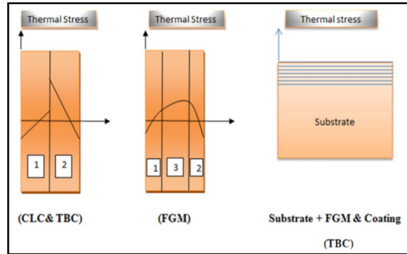
Figure 10. FGM and residual stresses
