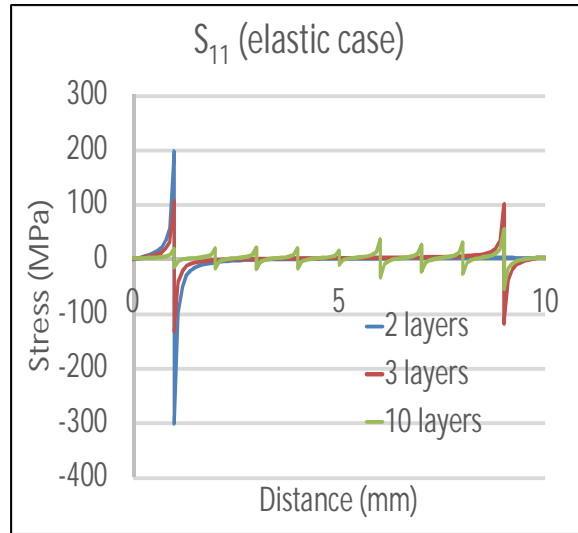
Figure 14 S_{11} (x dir.) Stress plot vs. thickness – elastic case
