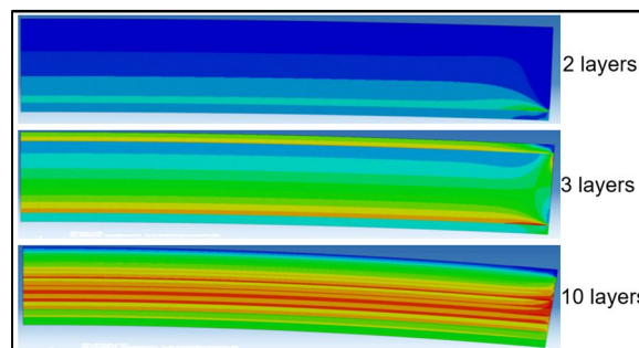
Figure 13. S_{vm} (Von Mises) Stress contours – elastic material properties.
