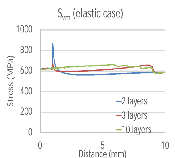
Figure 16 S_{vm} (Von Mises) Stress plot vs. thickness – elastic case
