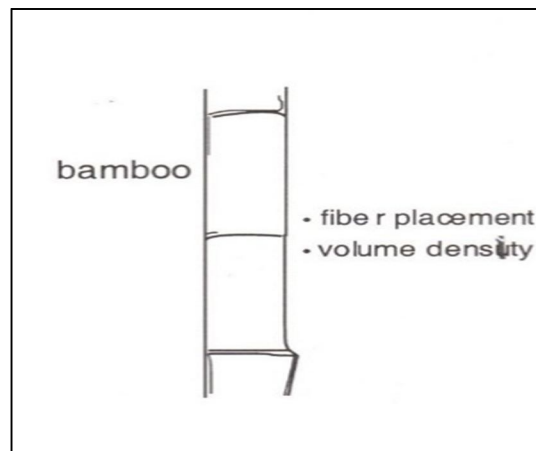
Figure 8. FGM in bamboo tree
