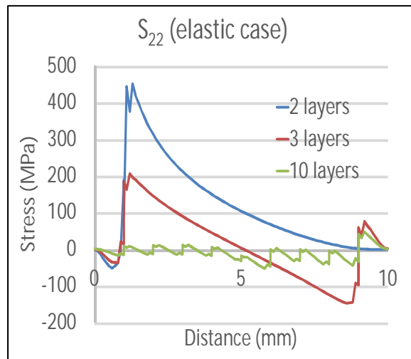
Figure 15 S_{22} (y dir.) Stress plot vs. thickness – elastic case
