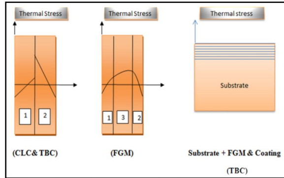
Figure 10. FGM and residual stresses
