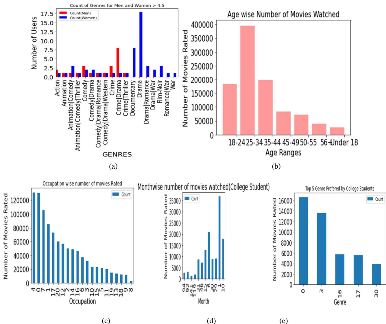
Figure 5- Figure 5(a) shows the count of Genres for men and women for several users > 4.5. Figure 5(b) shows the movie ratings by different age groups. Figure 5(c) shows the movie ratings by users of different occupations. Figure 5(d) shows the movies ratings for month-wise movies watched by college students. Figure 5(e) shows the movie ratings for top genres preferred by college students.
