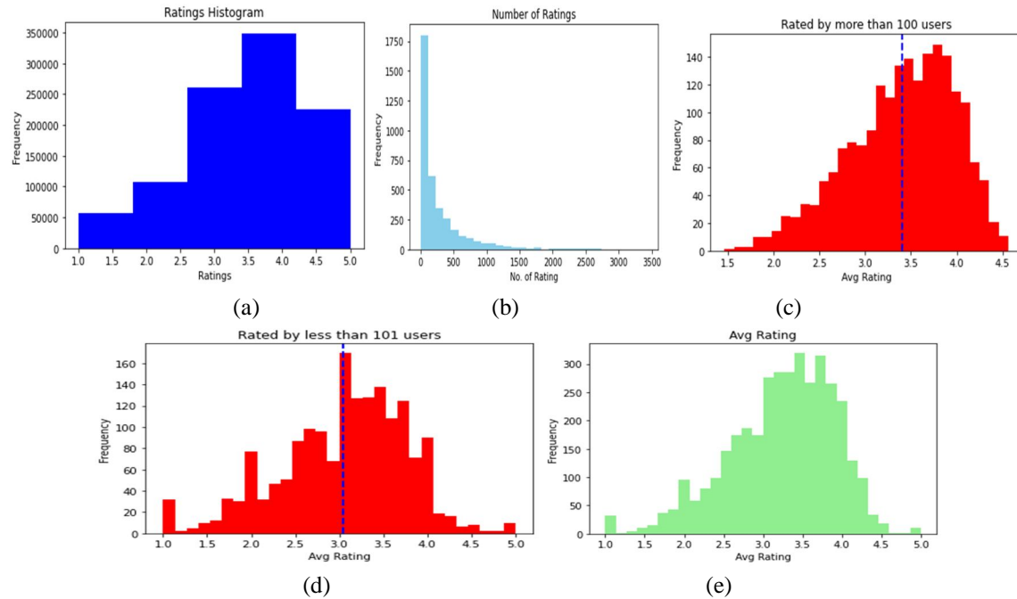
Figure 6- Figure 6(a) shows the rating histogram. Figure 6(b) illustrates the number of rating histograms. Figure 6(c) shows the average ratings for more than 100 users. Figure 6(d) represents the average ratings for less than 101 users. Figure 6(e) shows the average ratings done by users.
