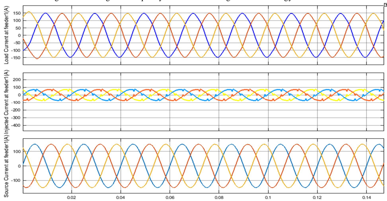
Fig. 7: Voltages and currents at feeder 1
