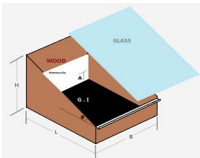
Figure. 1 Proposed Model of Solar Distillations System
