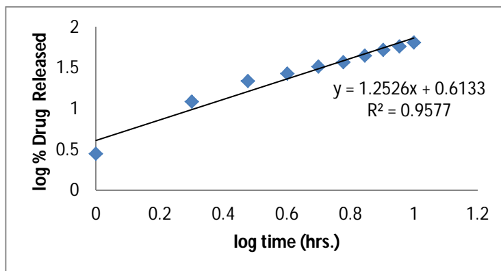
Fig. 14: Kinetic Drug Release Study of Pyridostigmine Nanoparticles Formulation (F2- Korsmeyer- peppas Model)
