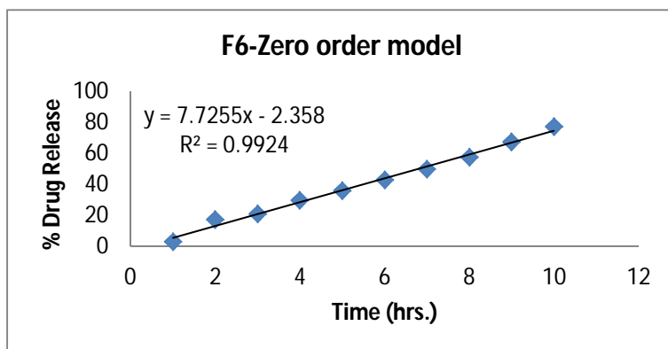
Fig. 16: Kinetic Drug Release Study of Pyridostigmine Nanoparticles Formulation (F6- Zero Order)
