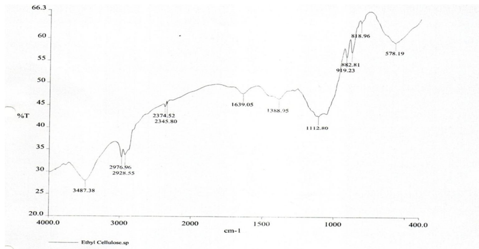
Fig. 3: FTIR of Ethyl cellulose
