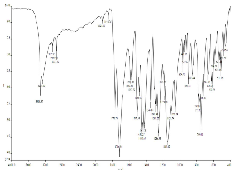
Fig. 2: FTIR of Pyridostigmine
