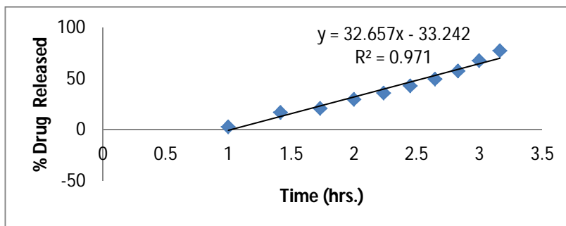
Fig. 19: Kinetic Drug Release Study of Pyridostigmine Nanoparticles Formulation (F6- Higuchi Model)
