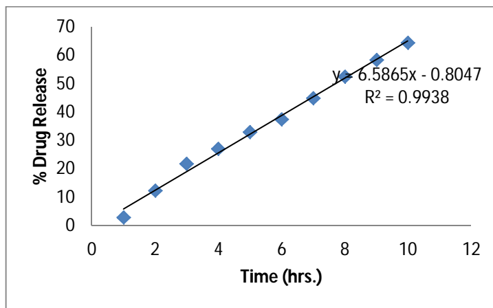
Fig. 12: Kinetic Drug Release Study of Pyridostigmine Nanoparticles Formulation (F2- Zero Order)
