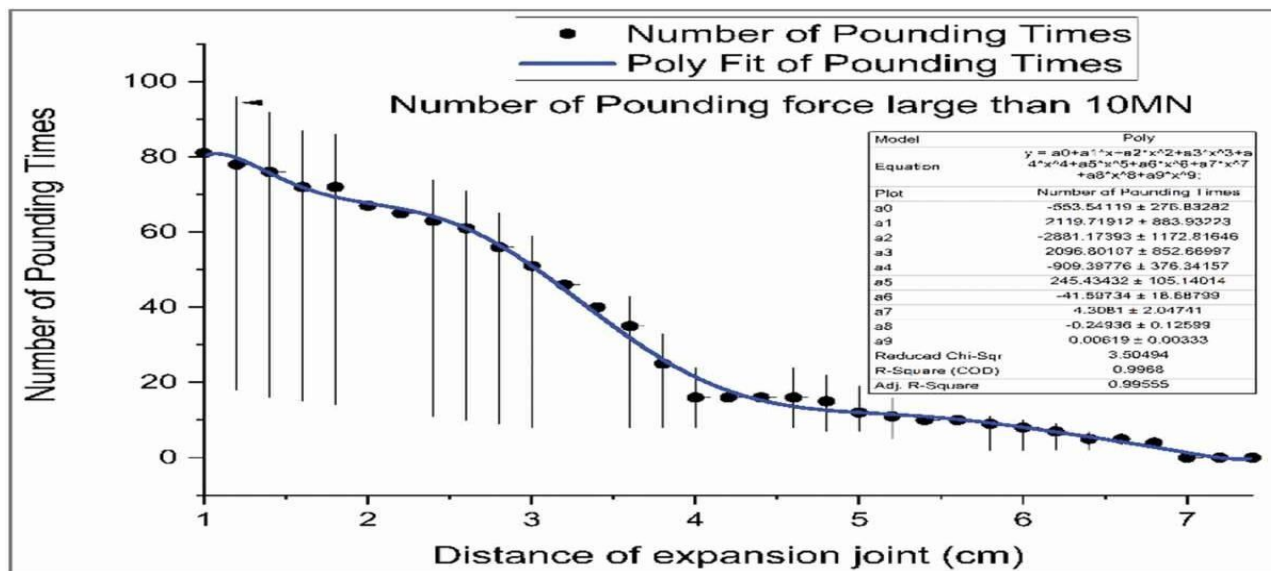
Figure. The relationship between collision times and the expansion joint width
