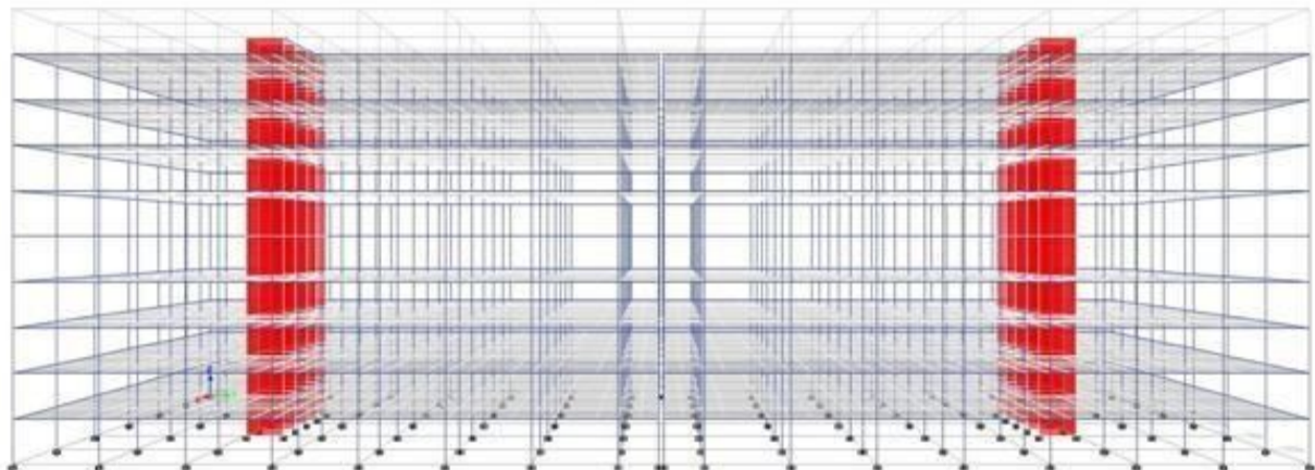
Figure: Elevation View of G+9 Structure of 90m slab length with expansion joint.
