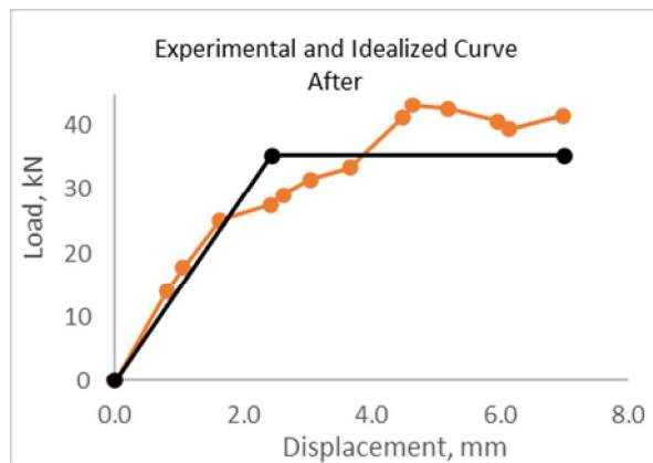
Figure 12: Bilinear Curve After Retrofitting
