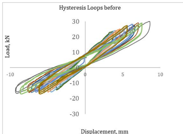
Figure 8: Hysteresis Curves before Retrofitting
