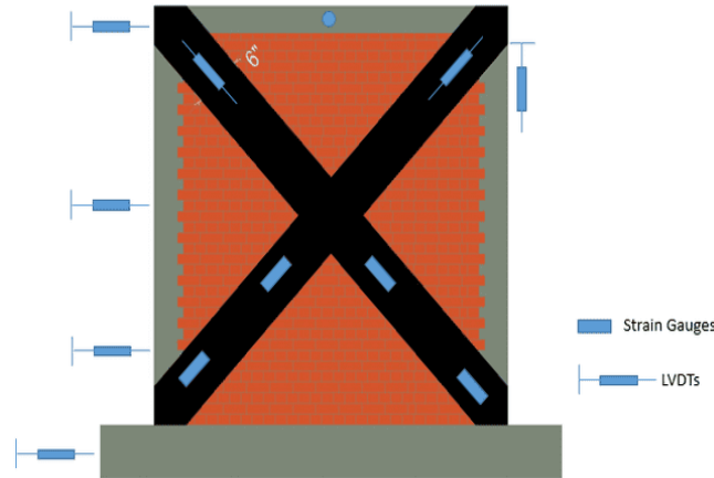
Figure 5. Instrumentation details
