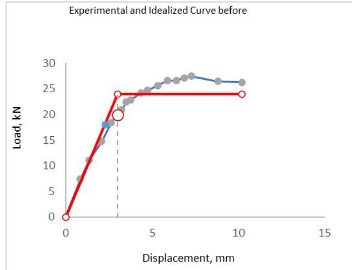
Figure 9: Bilinear Curve Before Retrofitting
