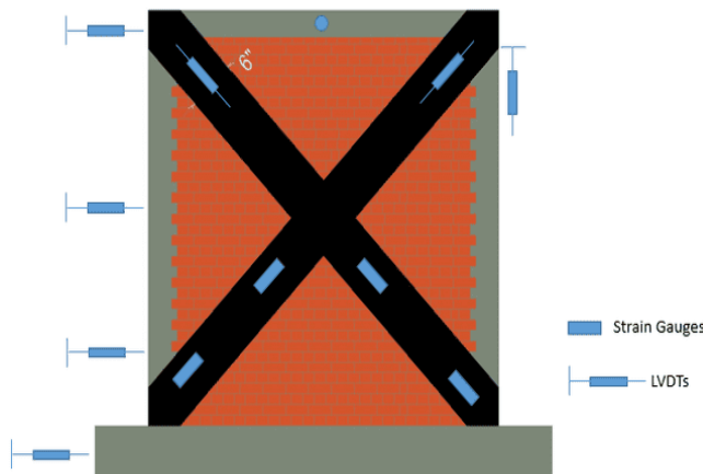
Figure 5. Instrumentation details
