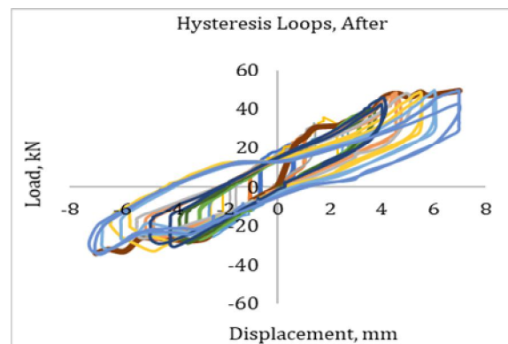
Figure 11. Hysteresis Curves after Retrofitting
