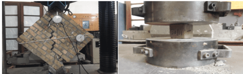
Figure 3. Diagonal Compression and Mortar Compressive Test
