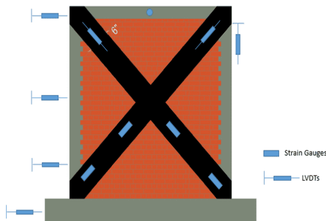
Figure 5. Instrumentation details
