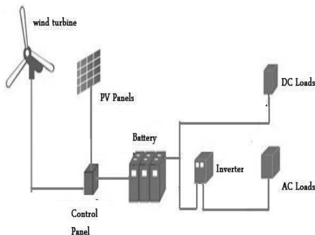
Fig.1. Hybrid Power Generation system
