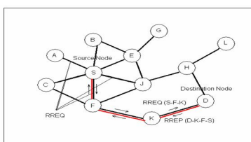
Figure 1 basic principle of Dynamic Source Routing
