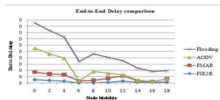
Figure4 Average end-to-end delay vs. node mobility
