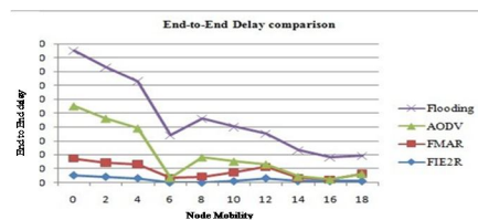
Figure4 Average end-to-end delay vs. node mobility
