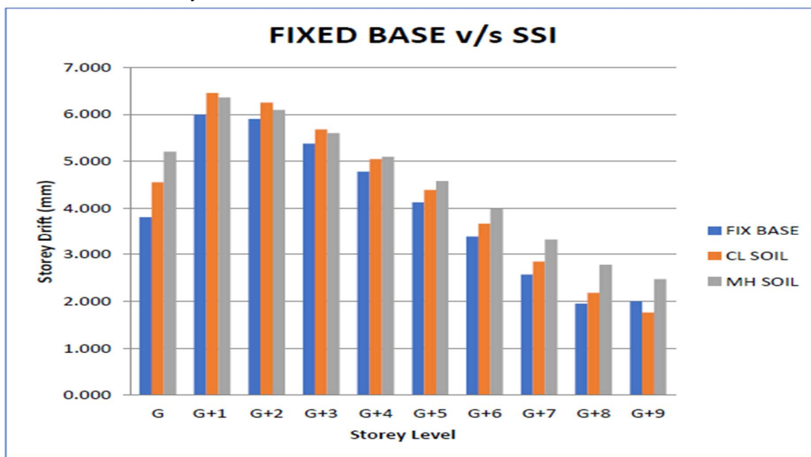
Fig -6: Storey Drift Comparison
