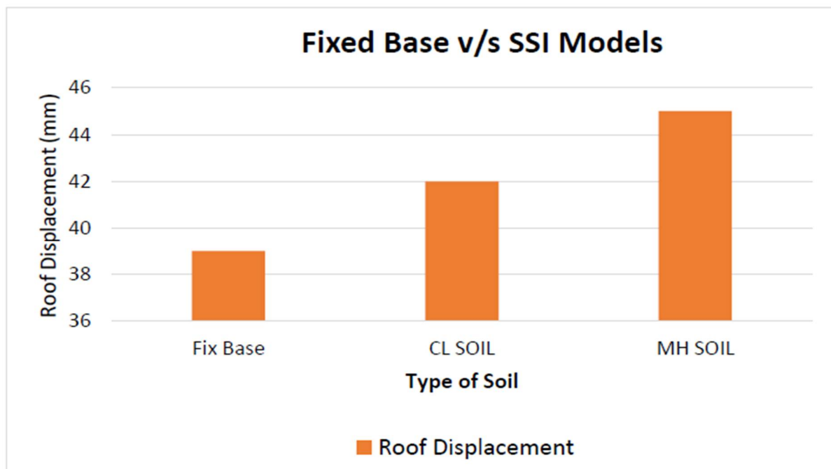
Fig -5: Roof Displacement Comparison
