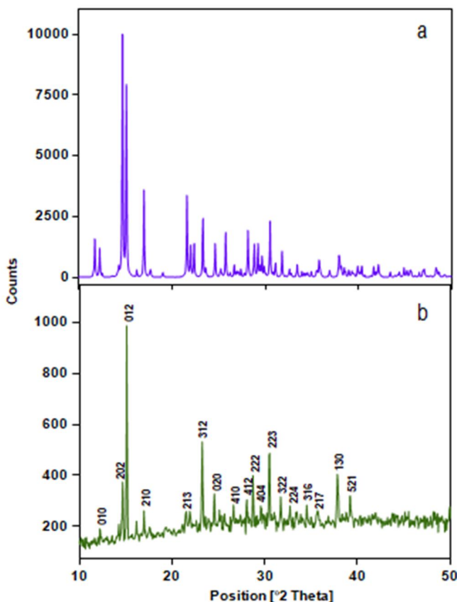
Fig. 5. Powder XRD patterns of HUCS: (a) simulated and (b) experimental.
