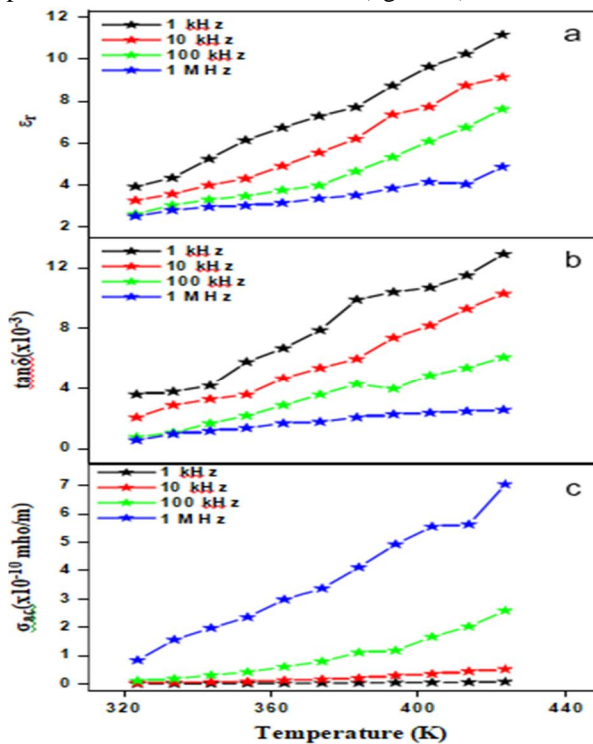
Fig. 10. Dielectric measurements for HUCS. (a) Plot of dielectric constant vs temperature (K), (b) Plot of dielectric loss vs temperature (K) and (c) Plot of AC electrical conductivity vs temperature (K)
