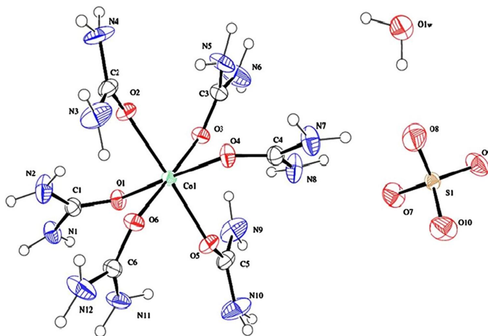
Fig. 3. ORTEP diagram of HUCS.
