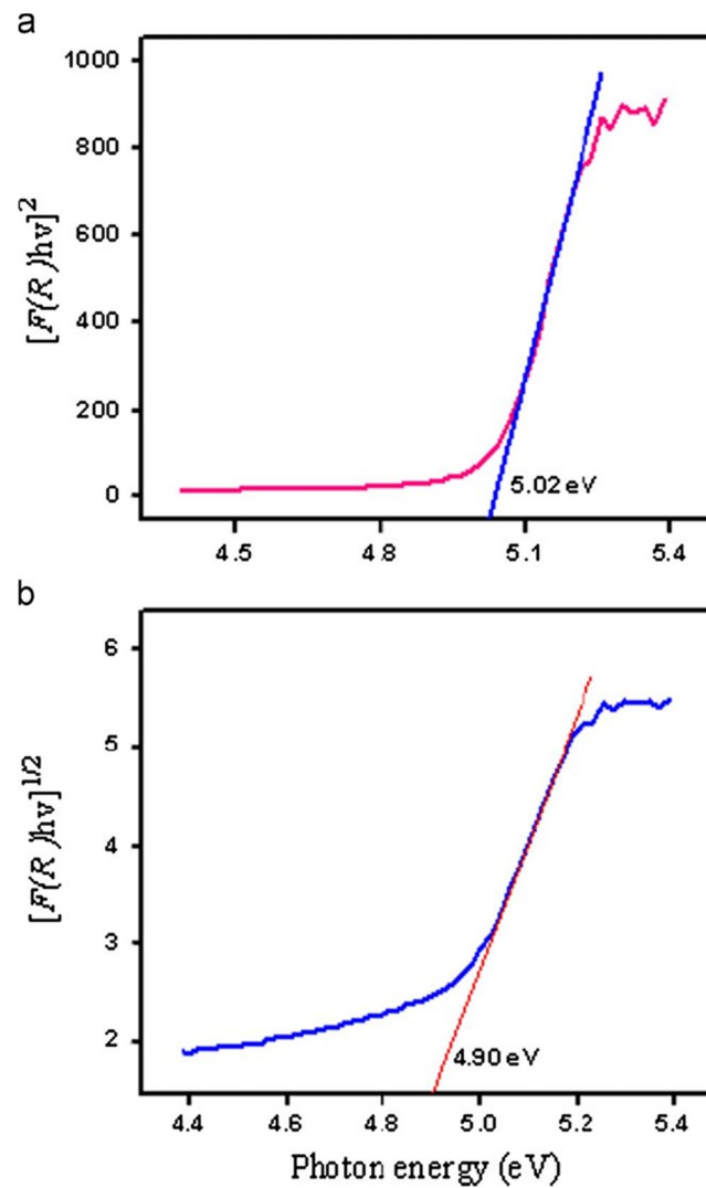
Fig. 7. Tauc's plot of HUCS: (a) direct (b) indirect.
