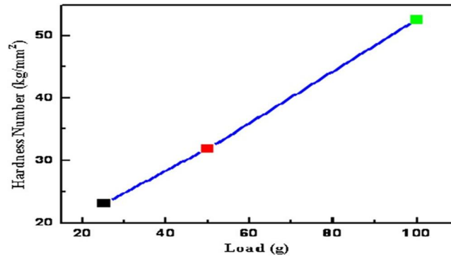
Fig. 9. The plot of Vickers hardness number (kg/mm 2 ) versus load (g) for HUCS.
