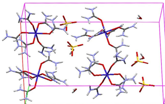
Fig. 4. Packing diagram of HUCS.
