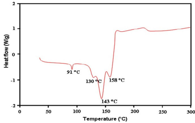
Fig. 8. DSC curve of HUCS.
