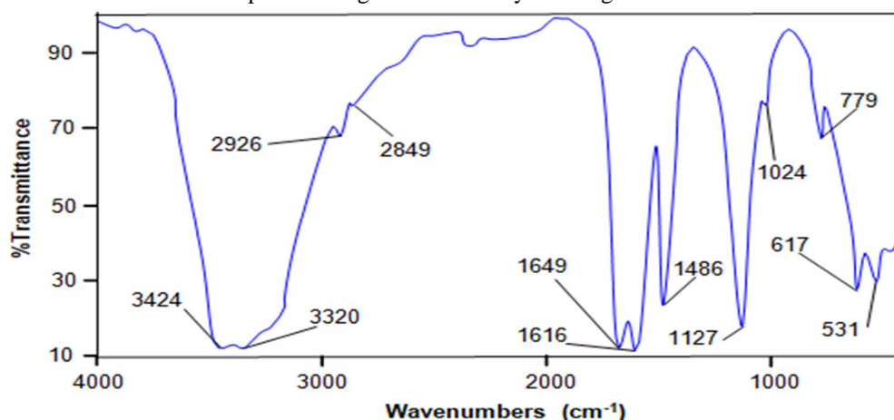
Fig. 2. FT-IR spectrum of HUCS.
