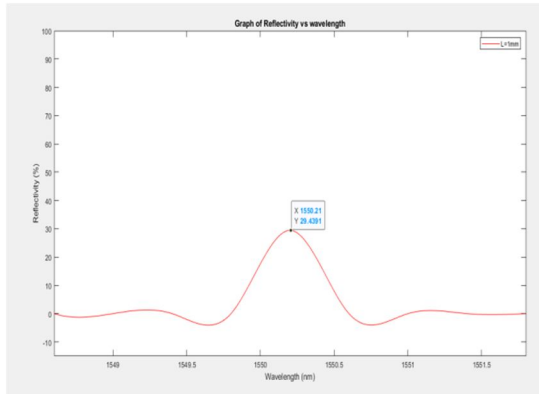
Figure 10 : The reflection spectrum of Fiber Bragg Grating with grating length, L = 1\text{mm} at refractive index change of \Delta n = 0.0003 with peak reflectivity, R = 29.44\%
