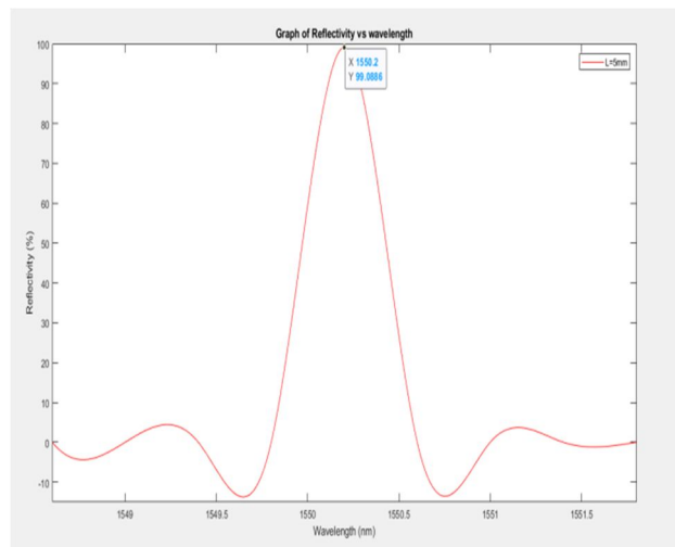
Figure 14 : The reflection spectrum of Fiber Bragg Grating with grating length, L = 5\text{mm} at refractive index change of \Delta n = 0.0003 with peak reflectivity, R = 99.08\%
