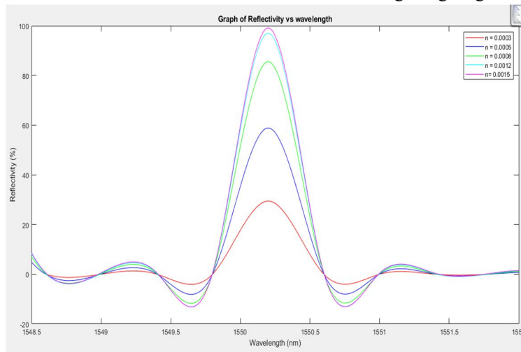
Figure 3 : The reflection spectrum of Fiber Bragg Grating with different refractive index change at grating length, L = 1mm
