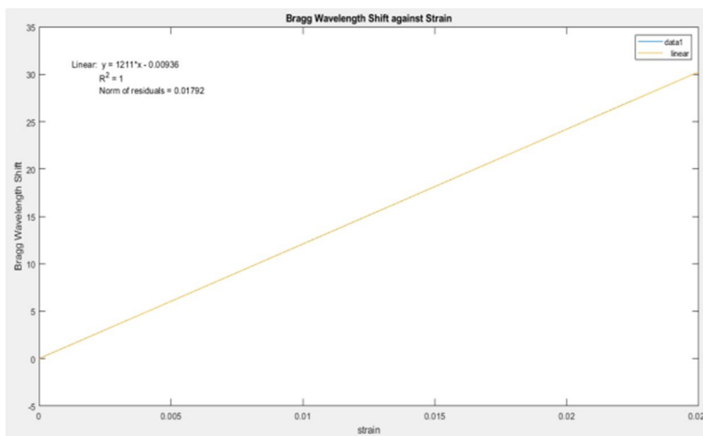
Figure 1 : Graph Bragg wavelength shift against strain in MATLAB
