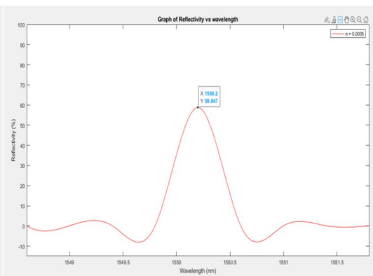
Figure 5 : The reflection spectrum of Fiber Bragg Grating for refractive index change of \Delta n = 0.0005 at grating length of L = 1mm with peak reflectivity, R = 58.85%
