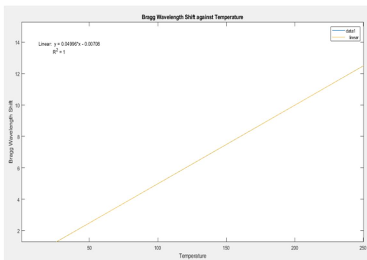
Figure 2 : Graph Temperature against Bragg Wavelength Shift in MATLAB
