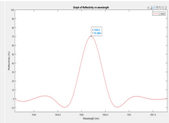
Figure 11 : The reflection spectrum of Fiber Bragg Grating with grating length, L = 2\text{mm} at refractive index change of \Delta n = 0.0003 with peak reflectivity, R = 70.31\%
