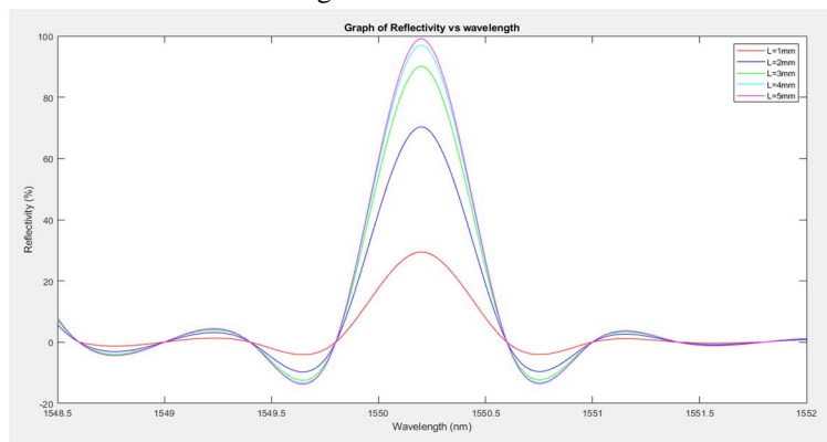
Figure 9 : The reflection spectrum of Fiber Bragg Grating with different grating length at refractive index change of \Delta n = 0.0003
