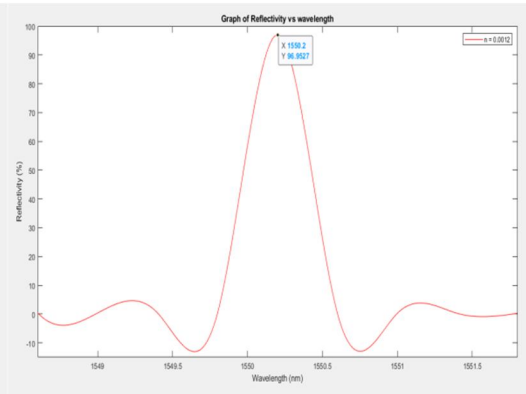
Figure 7 : The reflection spectrum of Fiber Bragg Grating for refractive index change of \Delta n = 0.0012 at grating length of L = 1\text{mm} with peak reflectivity, R = 96.95\%
