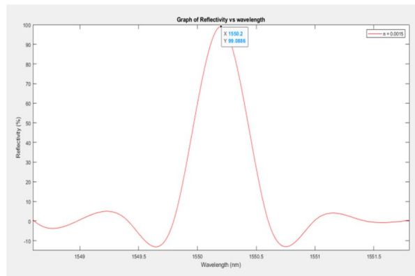
Figure 8 : The reflection spectrum of Fiber Bragg Grating for refractive index change of \Delta n = 0.0015 at grating length of L = 1\text{mm} with peak reflectivity, R = 99.09\%
