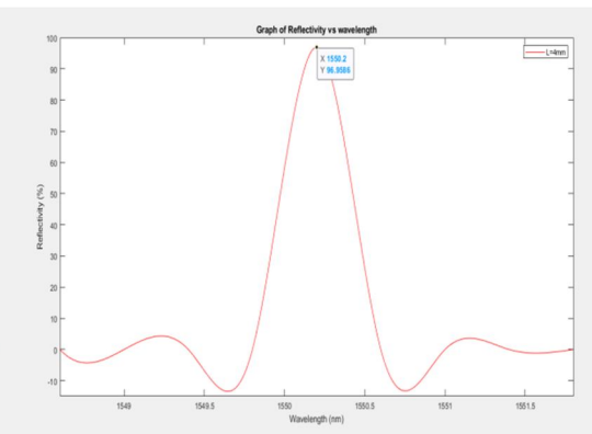
Figure 13 : The reflection spectrum of Fiber Bragg Grating with grating length, L = 4\text{mm} at refractive index change of \Delta n = 0.0003 with peak reflectivity, R = 96.96\%
