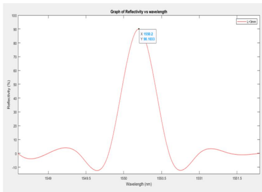
Figure 12 : The reflection spectrum of Fiber Bragg Grating with grating length, L = 3\text{mm} at refractive index change of \Delta n = 0.0003 with peak reflectivity, R = 90.10\%
