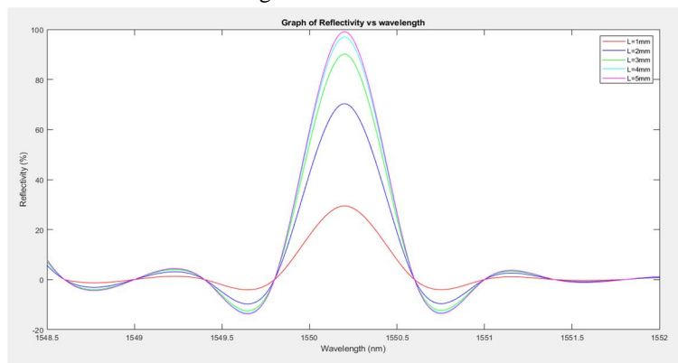
Figure 9 : The reflection spectrum of Fiber Bragg Grating with different grating length at refractive index change of \Delta n = 0.0003
