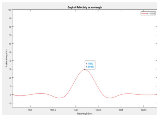
Figure 4 : The reflection spectrum of Fiber Bragg Grating for refractive index change of \Delta n = 0.0003 at grating length of L = 1mm with peak reflectivity, R = 29.45%
