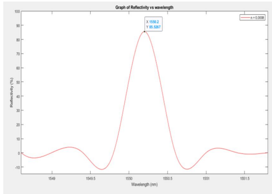
Figure 6 : The reflection spectrum of Fiber Bragg Grating for refractive index change of \Delta n = 0.0008 at grating length of L = 1\text{mm} with peak reflectivity, R = 85.53\%
