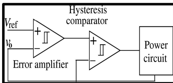
Fig.6 Voltage Hysteresis Control
