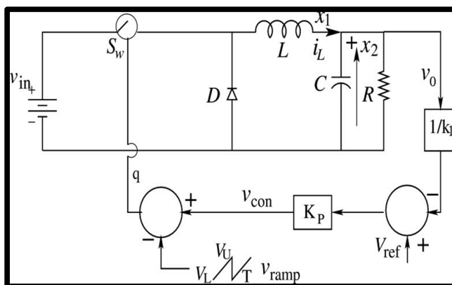
Fig.4 Block Diagram of Voltage Mode Controller
