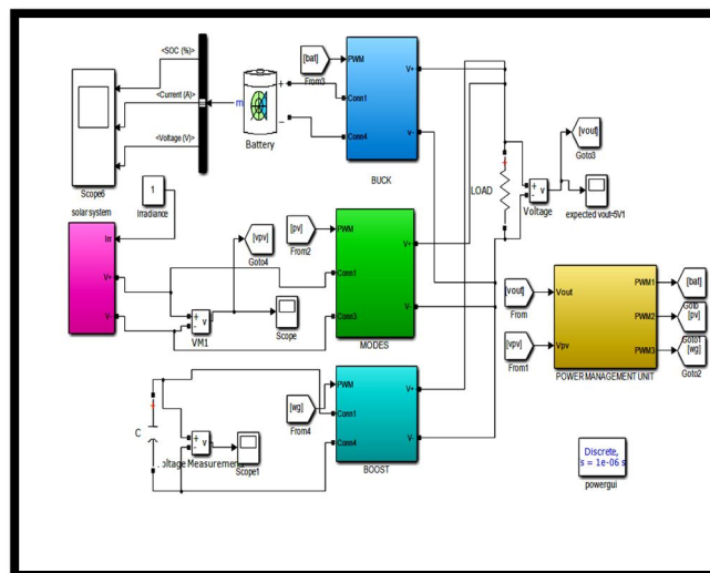
Fig.9 Simulation Model of the Proposed Work
