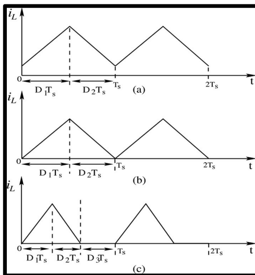
Fig.3 Inductor current waveform of PWM converter (a) CCM (b) boundary of CCM and DCM (c) DCM
