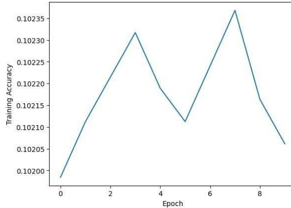
Fig.2.Training Accuracy Graph
