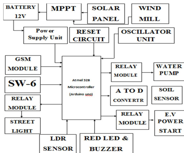
Fig.1: Block diagram for representation of system.
