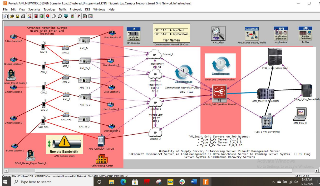
Figure 1 : SGIOT AIM Cloud Design Testbed
