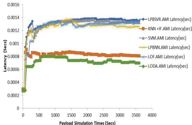
Fig 9 : Secure SG-IOT-CI-AMI Latency (secs)
