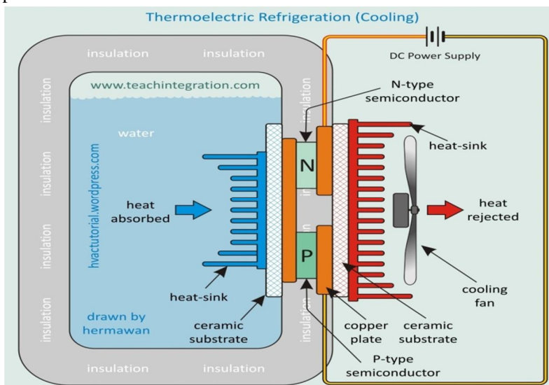
Fig.2 Schematic representation.
