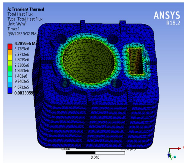
Fig.6 Fins Al 6061 materials total heat flux at 300 0 C transient
