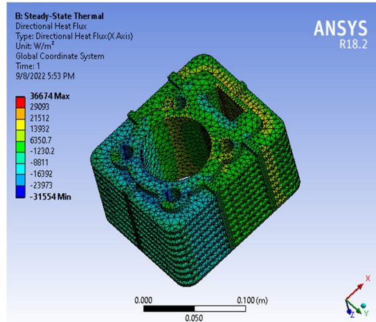
Fig.5 Fins Al 6061 Steady directional heat flux at 300 0 C
