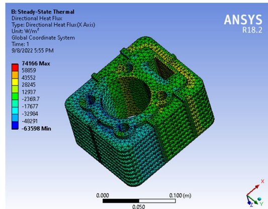
Fig. 11: Fins Al 6061 materials directional heat flux at 500°C steady
