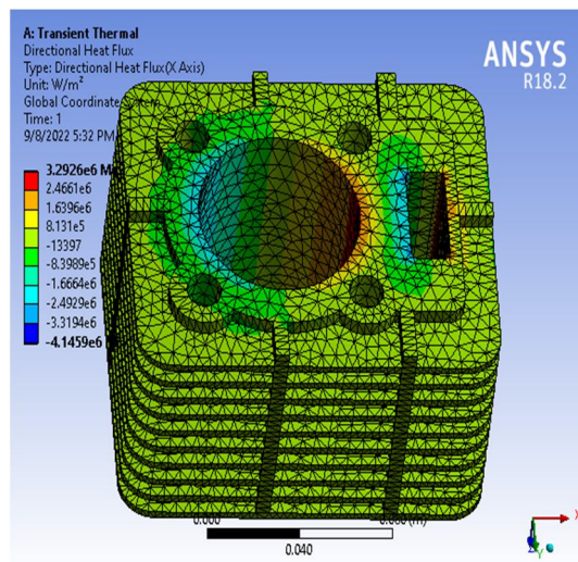
Fig.4 Fins Al 6061 materials directional heat flux transient at 300 °C
