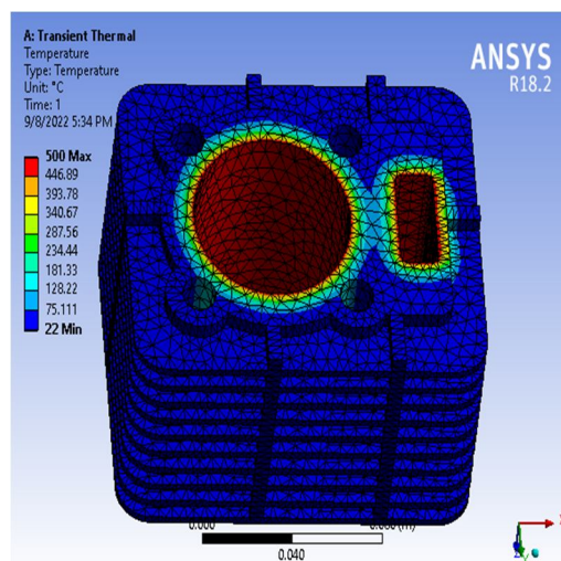
Fig. 14: Fins Al 6061 materials temperature at 500 0 C transient
