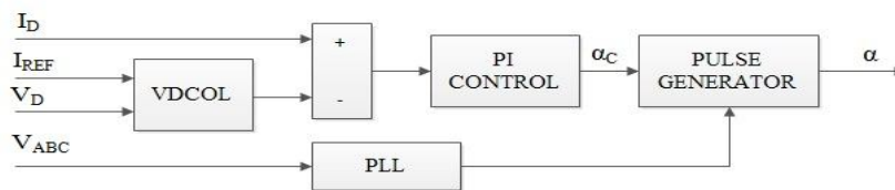
Fig. 2. Logic diagram of the rectifier control system model.
