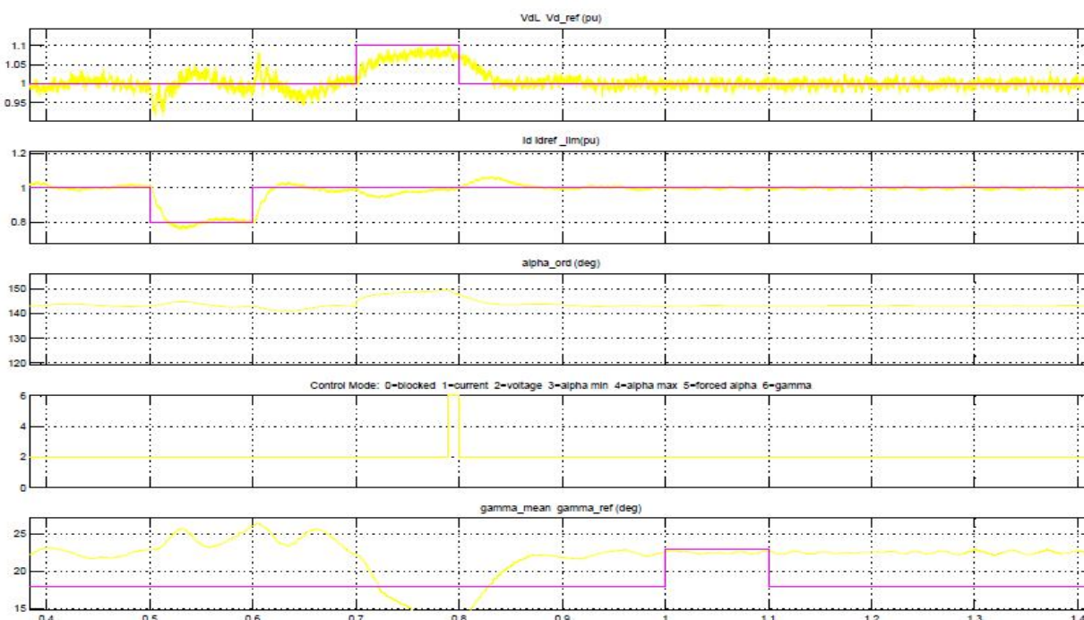
Fig. 5. Inverter DC quantities
