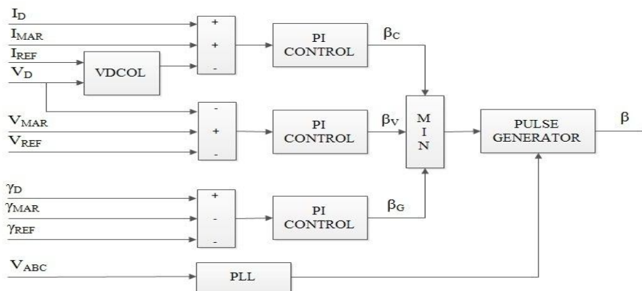
Fig 3. Logic diagram of the inverter control system model.
