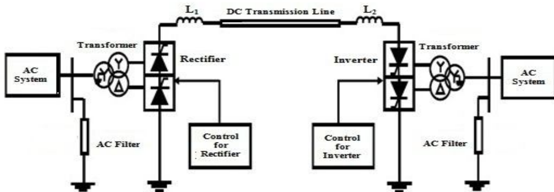
Fig. 1. The monopolar HVDC transmission system model
