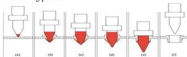
Fig -1: Process of Friction Drilling
