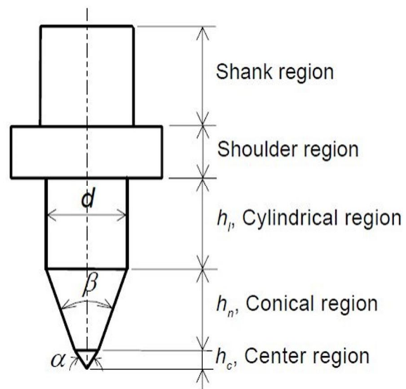
Fig -3: Different Regions in Friction Drill Tool
