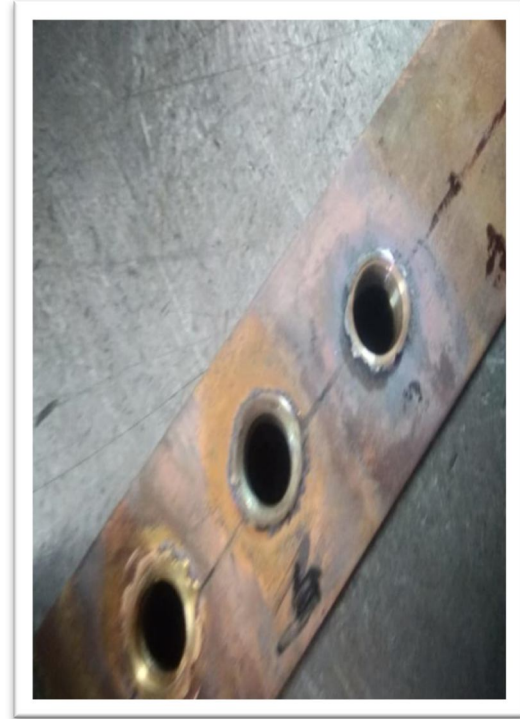
Fig-6: Holes made on Copper Plates By Friction Drilling.
