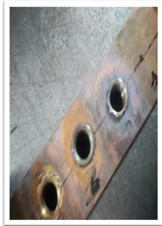
Fig-6: Holes made on Copper Plates By Friction Drilling.
