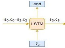
Figure 13: timestep t=3
