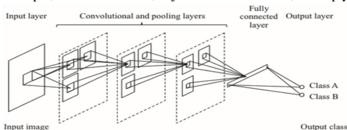
Fig. 2 Architecture of a CNN. The layers in the CNN are connected with local shift-invariant inter-connections (or convolution with a local kernel). The input and output of the CNN are images and class labels (e.g., Class A and Class B), respectively.
