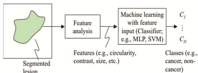
Fig. 1 Standard ML for classifying lesions (i.e., ML with feature input or feature-based ML) in the field of computer vision before the introduction of deep learning. Features (e.g., circularity, contrast, and effective diameter) are extracted from a segmented lesion in an image. Those features are entered as input to an ML model with feature input (classifier) such as a multilayer perceptron (MLP) and a support vector machine (SVM). The output of the classifier consists of class categories such as cancer or non-cancer.
