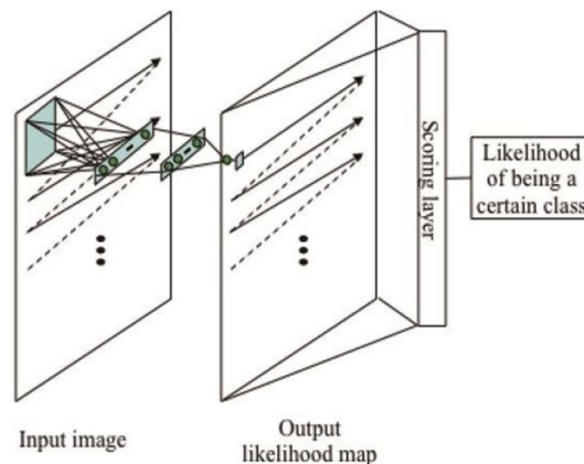
Fig. 6 Architecture of an MTANN consisting of an ML model (e.g., linear-output-layer ANN regression) with sub region (or image patch, local kernel) input and single-pixel output. The entire output image representing a likelihood map is obtained by scanning with the input sub region of the MTANN in a convolutional manner on the entire input image. A scoring layer is placed in the end to convert the output likelihood map into a single score that represents the likelihood of being a certain class for a given input image.
