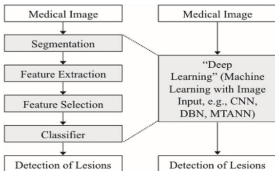
Fig. 4 Changes in ML approaches before and after the introduction of ML with image input (image-based ML) including “deep learning”. Compared to ML with feature
