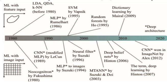
Fig. 5 The history of ML in the fields of computer vision and medical imaging. There are two distinct ML approaches in these fields. Before the popularity of “deep learning” starting in 2013, ML with feature input (feature-based ML) was dominant in the fields. After that, ML with image input (image-based ML) including deep learning gained enthusiastic popularity, but it has a long history
