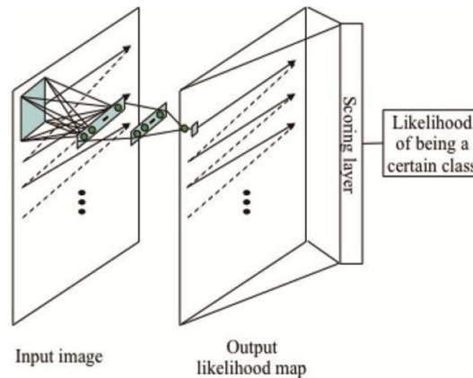
Fig. 6 Architecture of an MTANN consisting of an ML model (e.g., linear-output-layer ANN regression) with sub region (or image patch, local kernel) input and single-pixel output. The entire output image representing a likelihood map is obtained by scanning with the input sub region of the MTANN in a convolutional manner on the entire input image. A scoring layer is placed in the end to convert the output likelihood map into a single score that represents the likelihood of being a certain class for a given input image.
