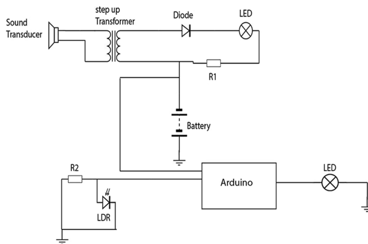
Fig 2: Circuit Diagram
