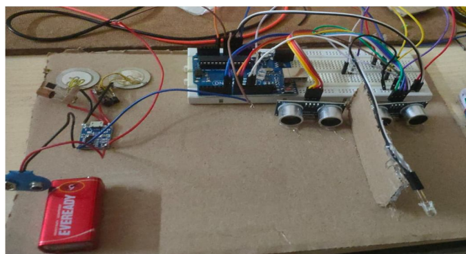
Fig 5: Implementation diagram
