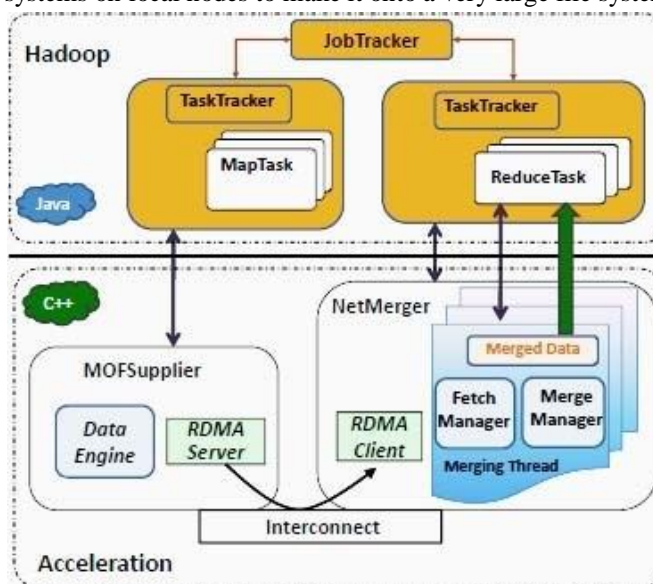
Fig 2: Hadoop structure
