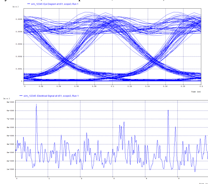
Graph of Electrical Signal And Eye Pattern (for D = 16 \text{ ps/nm/km} , \alpha = 0.2 \text{ dB/km} ):
