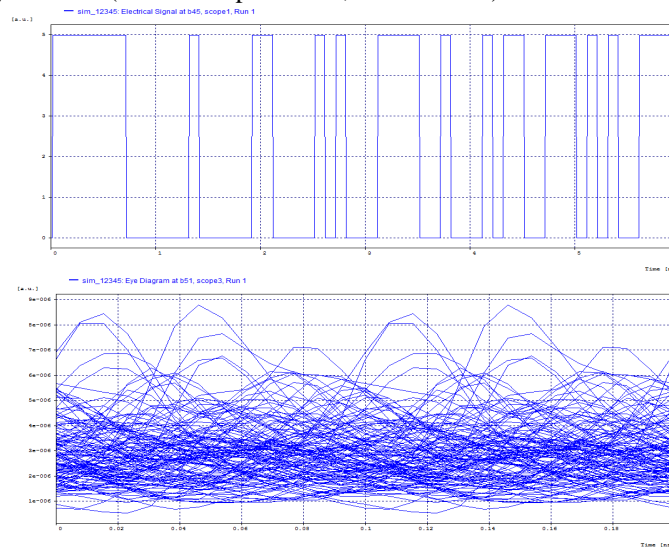
Graph of Electrical Signal And Eye Pattern (for D = 16 \text{ ps/nm/km} , \alpha = 0.5 \text{ dB/km} ):
