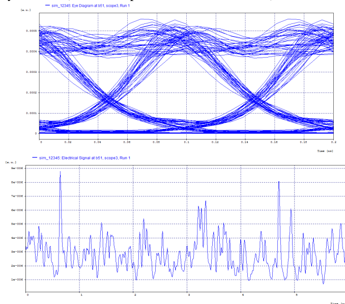
Graph of Electrical Signal And Eye Pattern (for D = 16 \text{ ps/nm/km} , \alpha = 0.2 \text{ dB/km} ):
