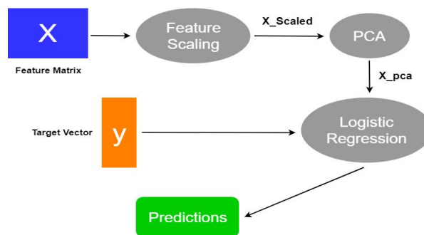
Steps of applying logistic regression with PCA
