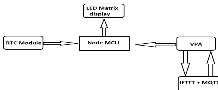
Fig. 4: The Block diagram
