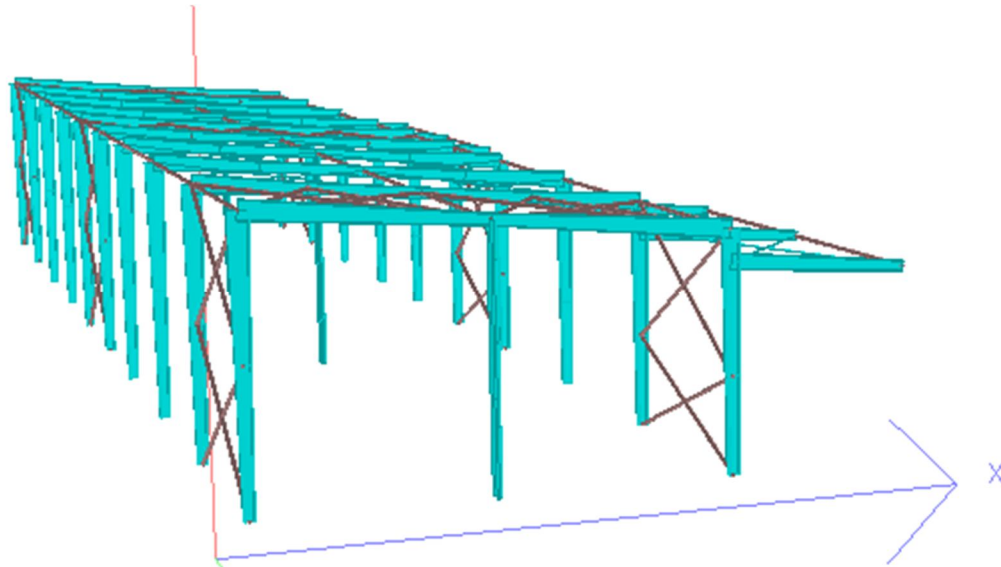
Figure 2 – 3D view
