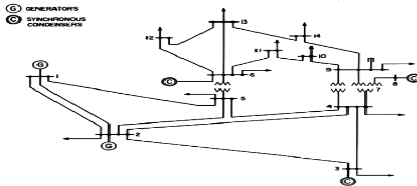
Fig1: IEEE-14 bus system
