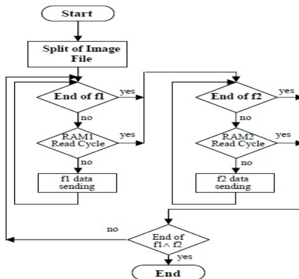
Fig 3: Two Levels System Flow Chart
