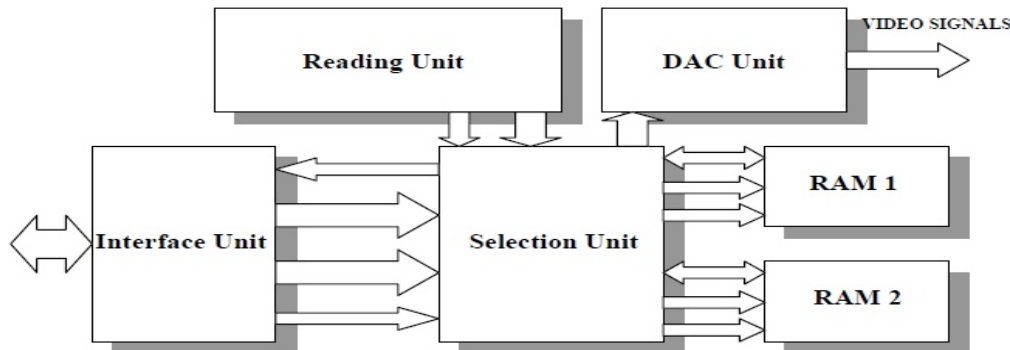
Fig 2: Two Levels System Block Diagram
