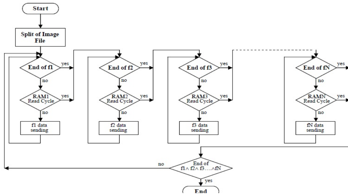
Fig 5. N levels system flow chart
