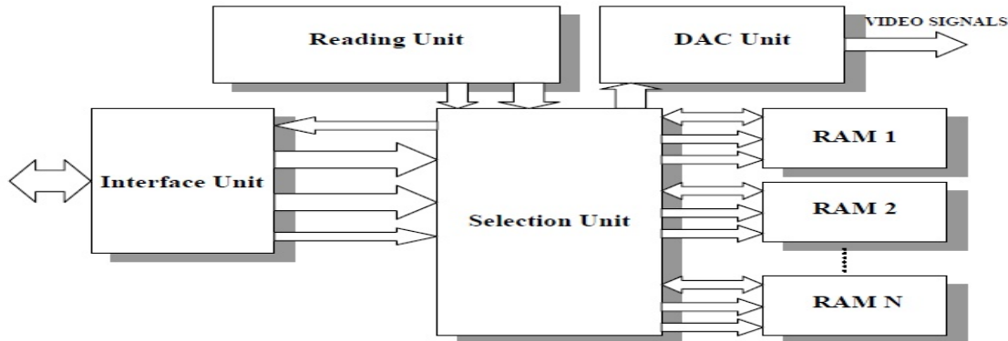
Fig 4: N Levels System Block Diagram
