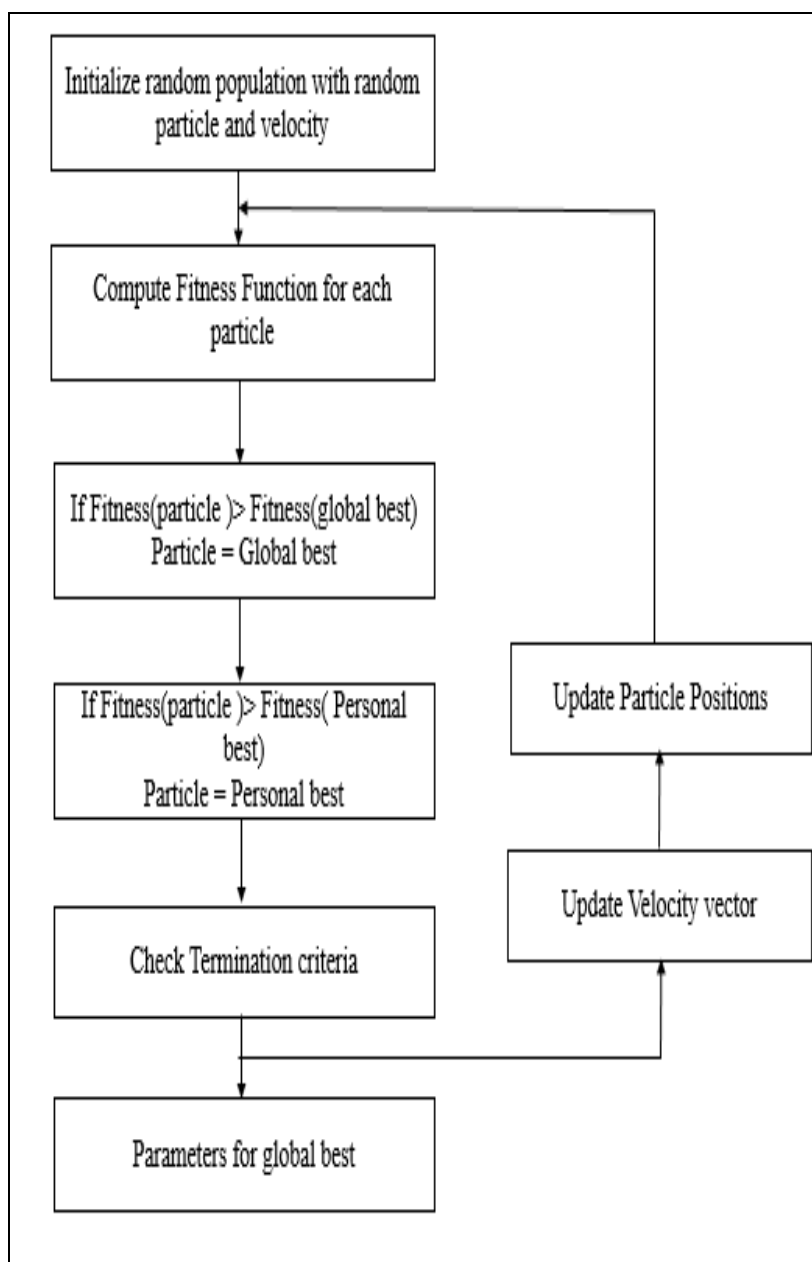
Figure 3 General Approach for particle swarm optimization
