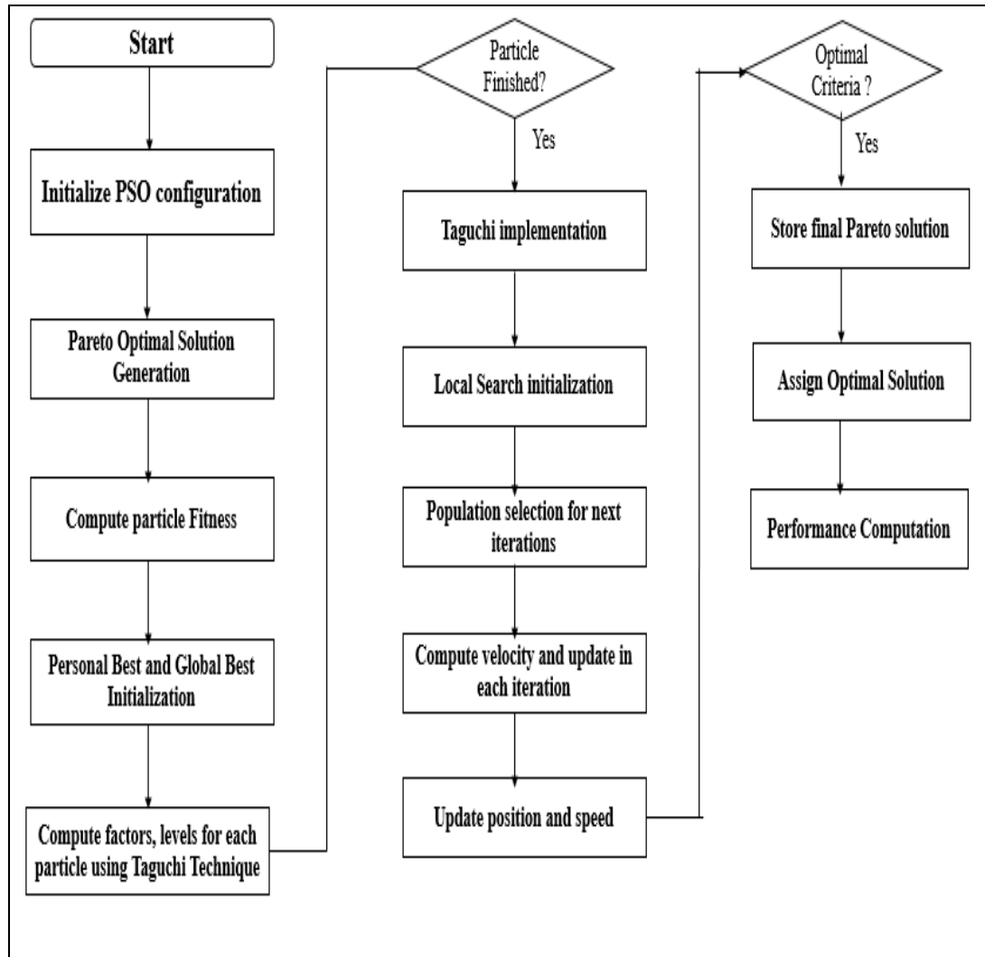
Figure 5 Taguchi and PSO implementation with optimal solution
