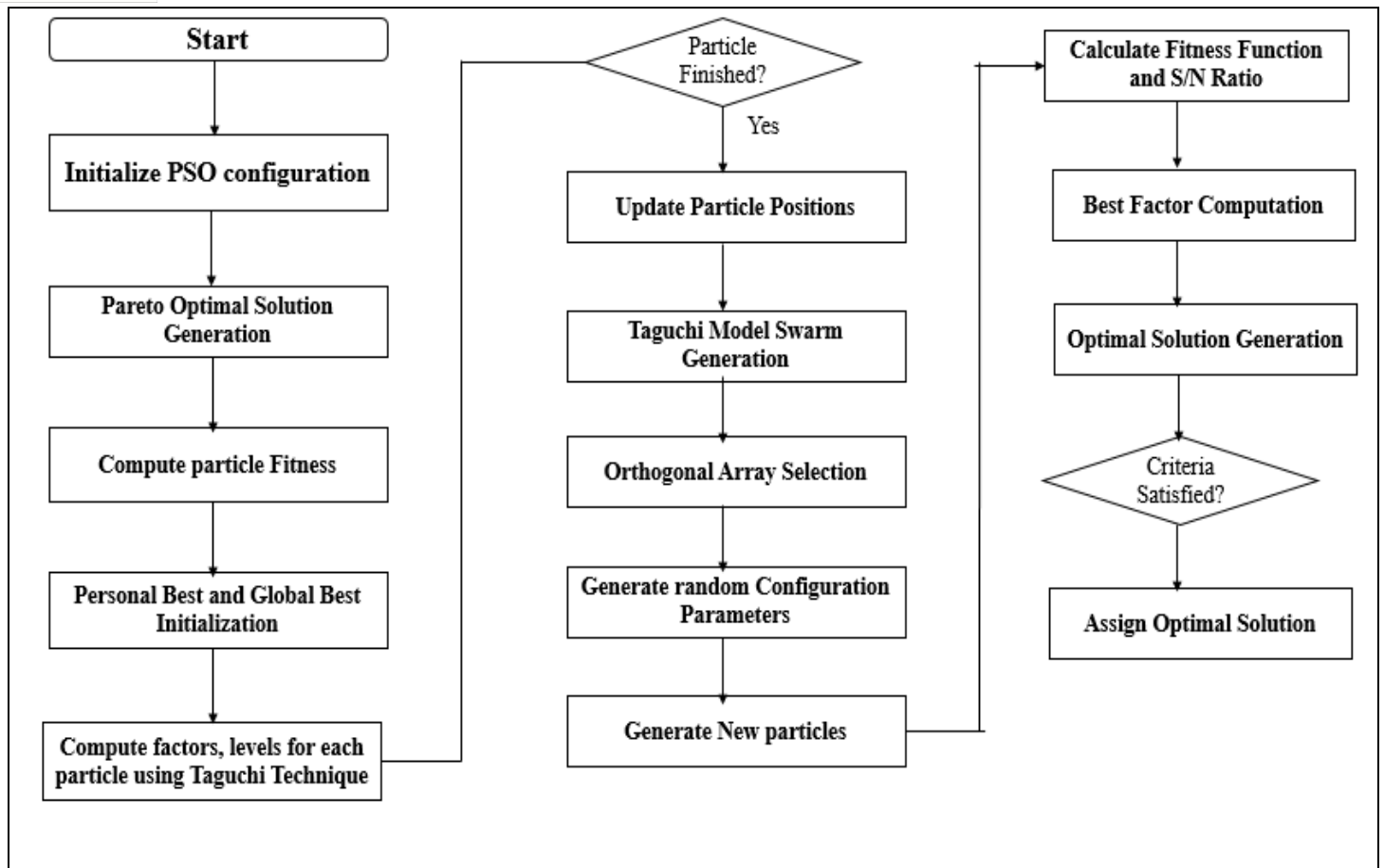
Figure 4 Taguchi and PSO implementation without optimal solution
