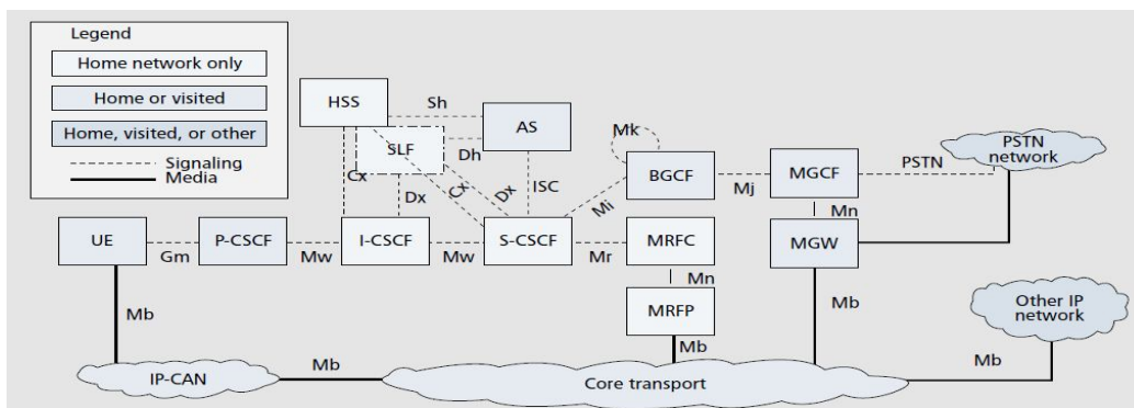
Figure 4 IMS functional entities and reference points.
