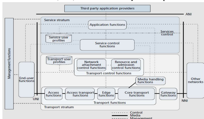
Figure 2 NGN architecture overview
