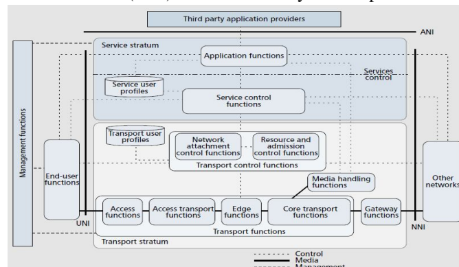
Figure 2 NGN architecture overview
