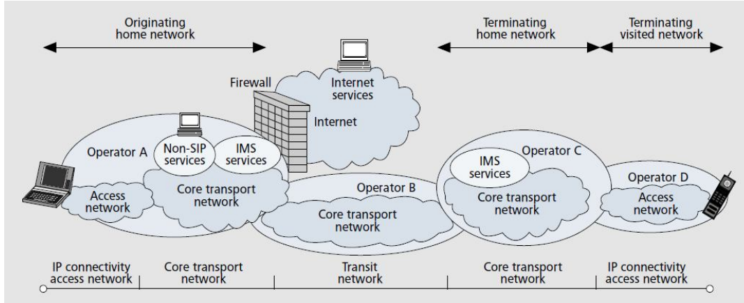
Figure 3 Network partitioning.
