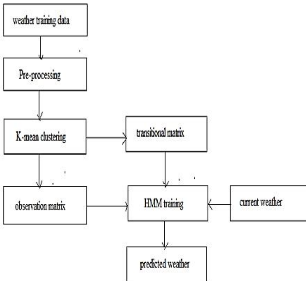
Figure 4: A weather forecasting technique using K-mean clustering
