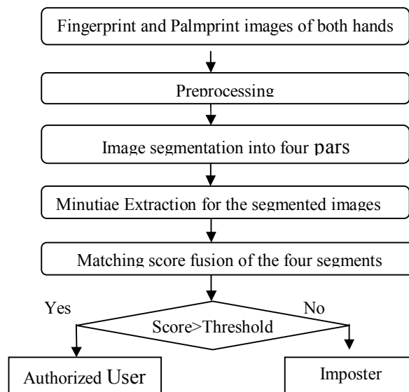
Fig.4. Flow Chart of the proposed Matching System.
