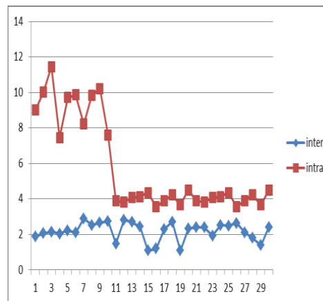
Fig.6. Matching Score of the Proposed System
