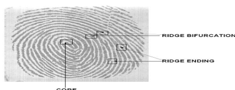
Fig.1. Fingerprint Image
