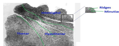
Fig.2. Palmprint Image
