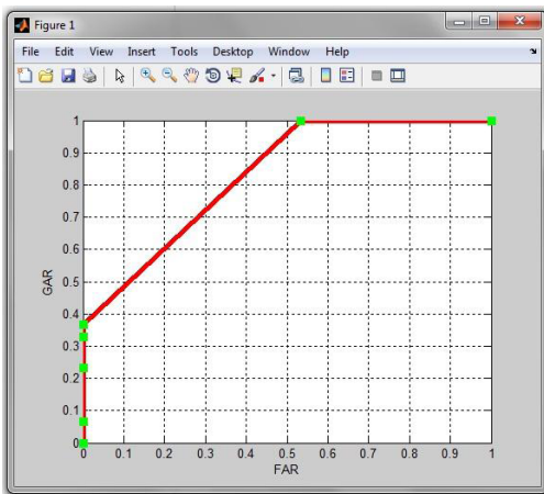
Fig.5. GAR and FAR Graph
