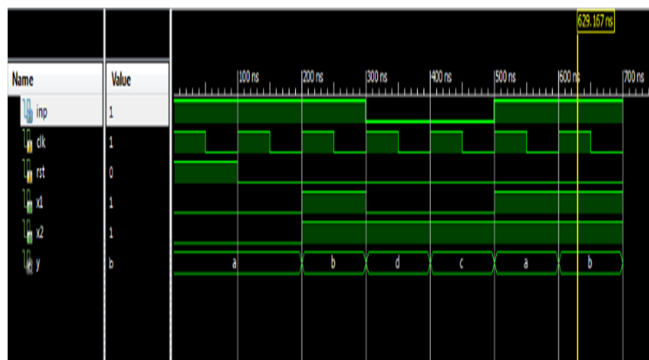
Figure: 11 Simulation results of convolutional encoder.
