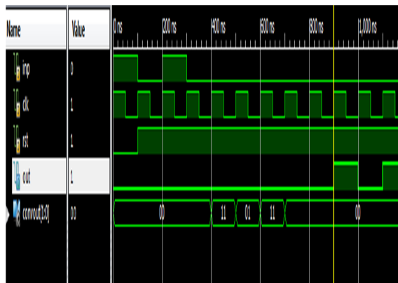
Figure: 15 Simulation result of modified viterbi decoder.
