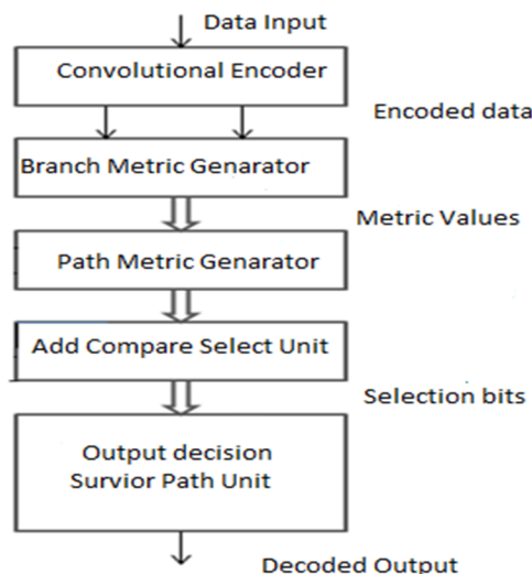
Figure: 10 Flowchart of the convolutional encoder and viterbi decoder
