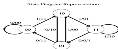
Figure: 3 State diagram of convolutional encoder.
