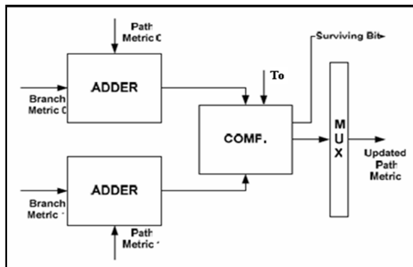
Figure: 8 Add Compare Select Unit.
