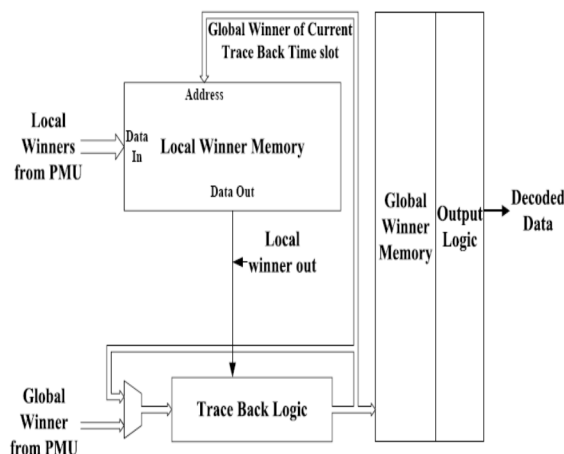
Figure: 9 Survivor path unit with path memory
