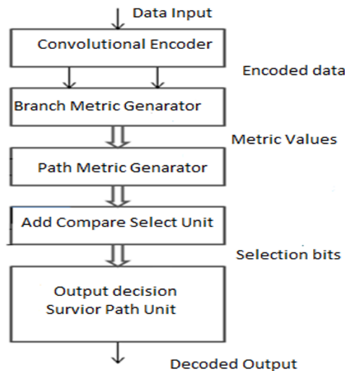
Figure: 10 Flowchart of the convolutional encoder and viterbi decoder
