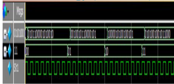
Figure.12. Simulation result of Branch Metric Unit.
