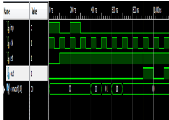
Figure: 15 Simulation result of modified viterbi decoder.
