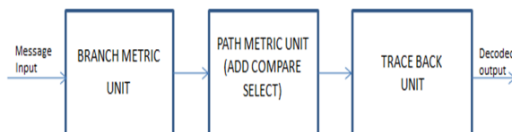
Figure:6 Block diagram of viterbi decoder.
