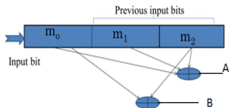
Figure: 2: Convolutional encoder.
