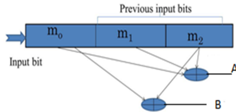
Figure: 2: Convolutional encoder.
