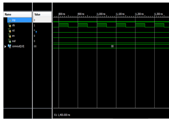
Figure: 14 Simulation results of viterbi decoder.
