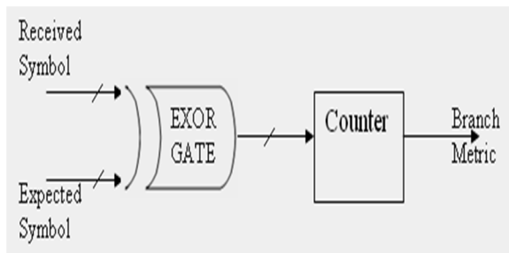
Figure: 7 Branch metric calculation
