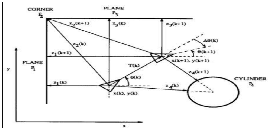
Fig.1. Localization by concurrent observation of several geometric beacons
