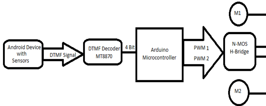
Figure 3.2: Robot motion Block Diagram
