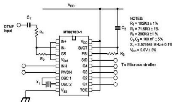
Figure 3 .4: The schematic diagram for MT8870
