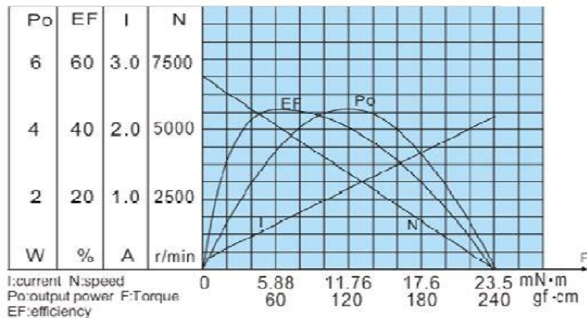
Figure 3.3: SPG30E-30K DC Motor characteristics
