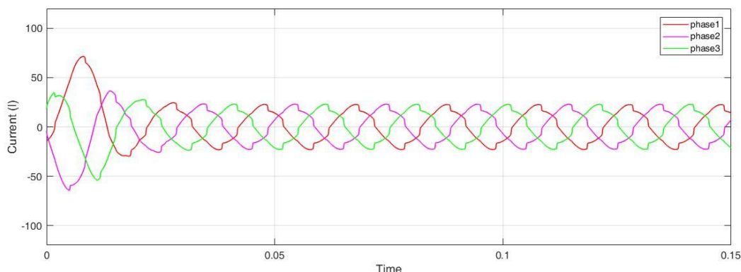
Fig. 6 Voltage and Current Waveform with Active Harmonic Filters.
