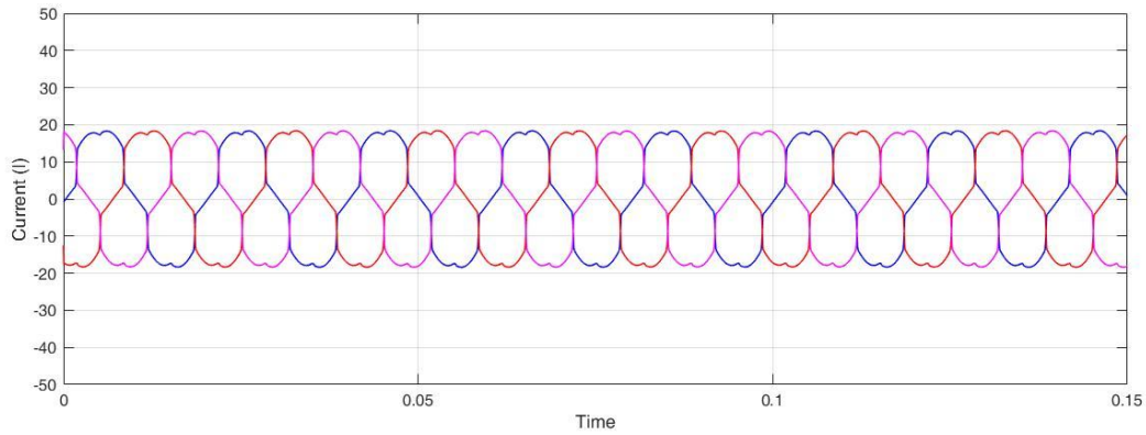
Fig. 4 Voltage and Current Waveform with Passive Harmonic Filters.
