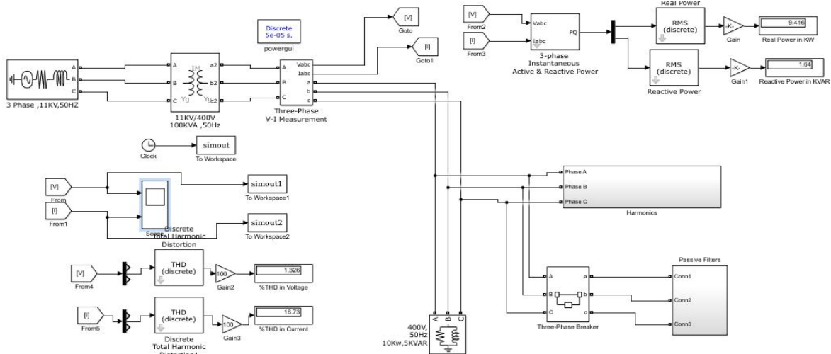
Fig. 3 MATLAB based model with Passive Filters.
