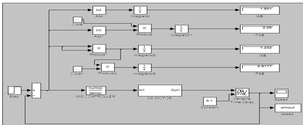
Figure 12: Simulink Model of the DC Servomotor with IMC Controller.
