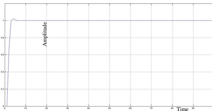
Figure 6 : Chien-Hrones-Reswick PID Response
