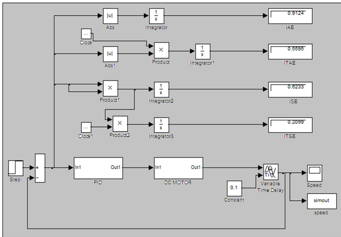
Figure 3: Simulink Model of the DC Servomotor with PID Controller
