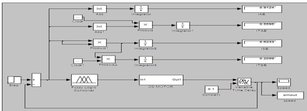
Figure 8: Simulink Model of the DC Servomotor with Fuzzy Logic Controller
