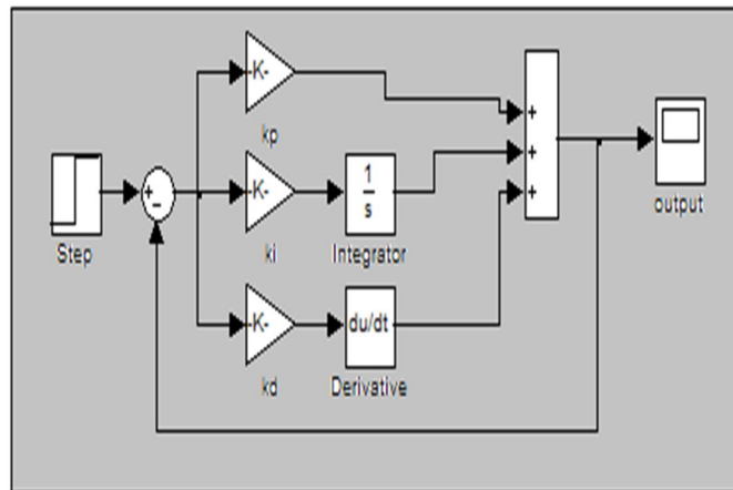
Figure 2: Block Diagram of PID controller
