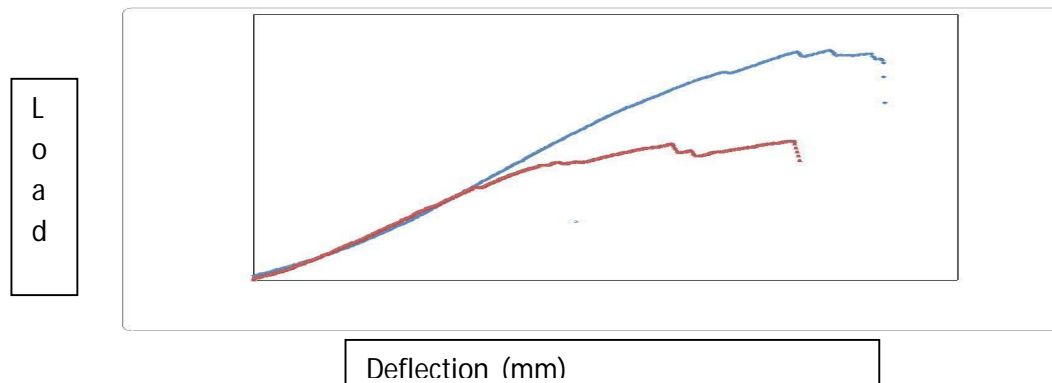
Figure 7: Load-deflection of ILSS test.
