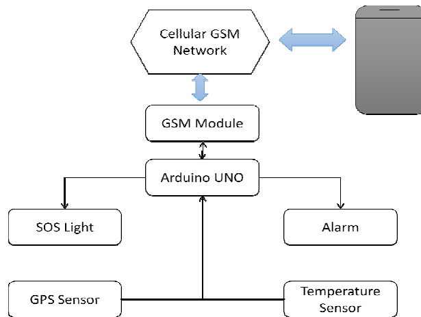
Fig. 1 System overview of the wearable device.
