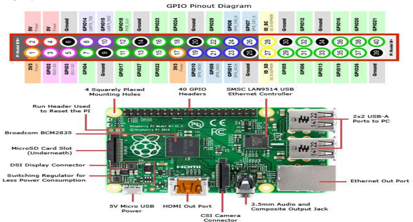
Fig.2 Pin Diagram of Raspberry Pi.
