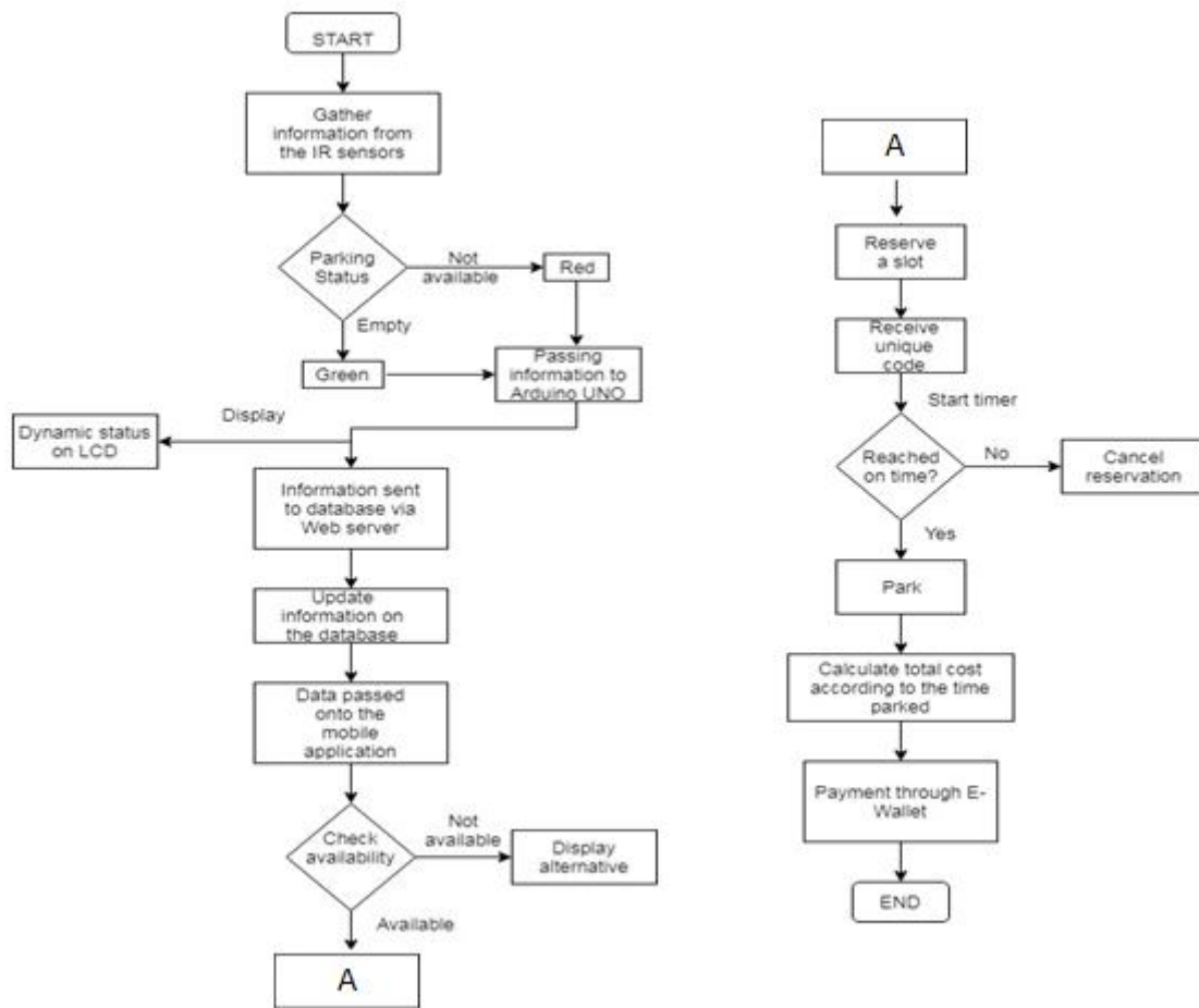
Fig.6. System Flowchart
