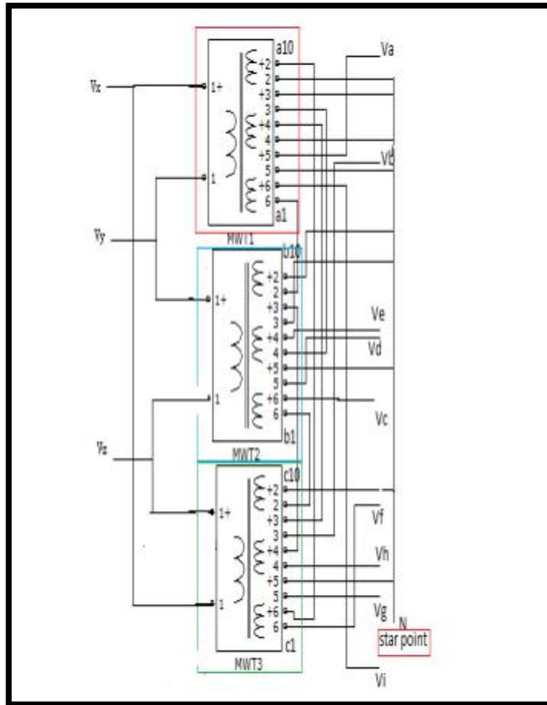
Fig V proposed winding arrangement (delta-star)
