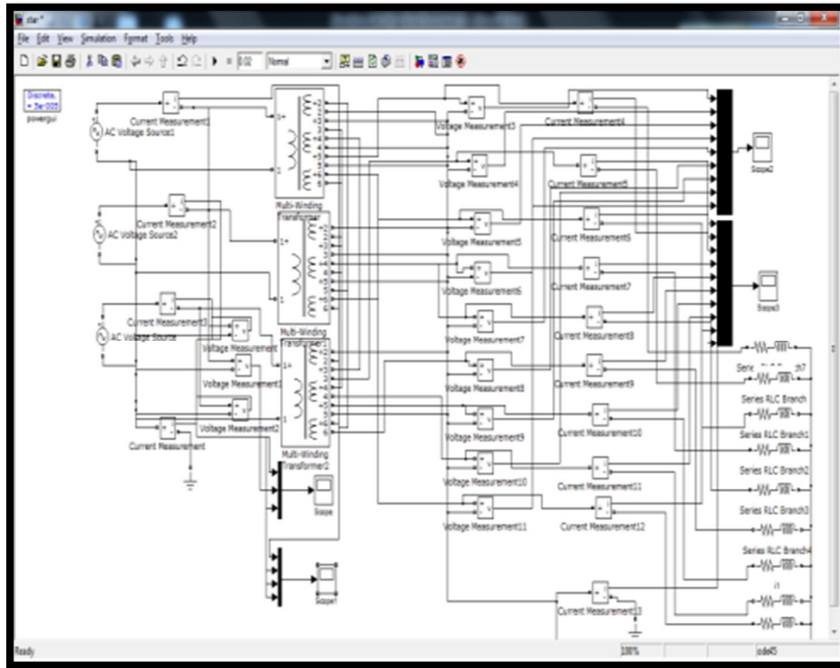
Fig VII shows the simulation circuit for star-star connection
