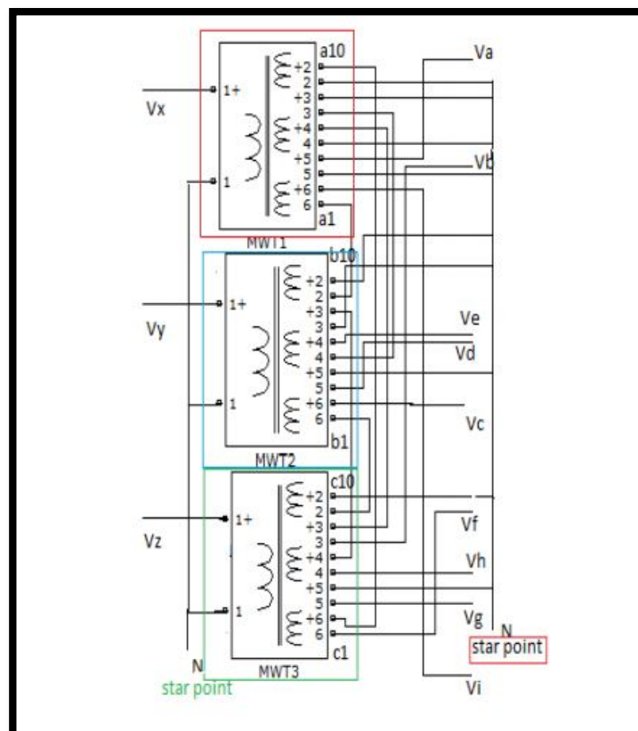
Fig: II proposed winding arrangement (star-star)
