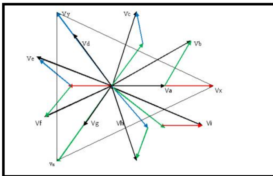
Fig VI Phasor diagram of the proposed transformer connection (delta-star).
