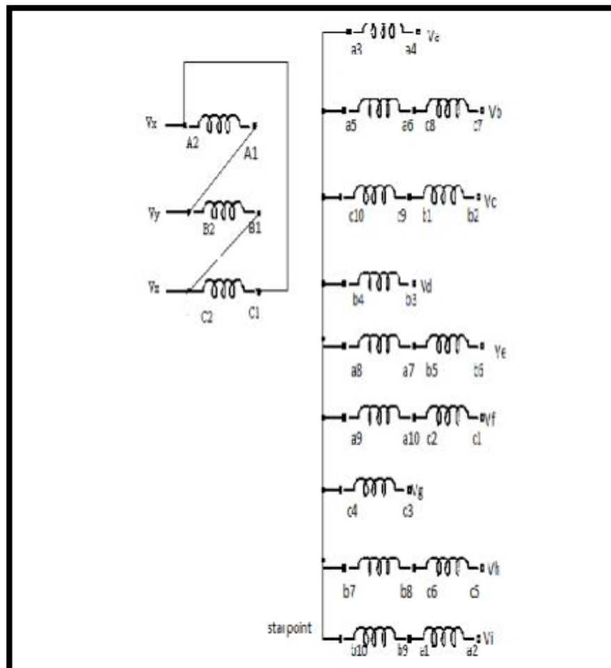
Fig IV Proposed transformer winding connection (delta-star).
