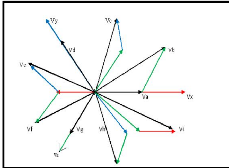
Fig III. Phasor diagram of the proposed transformer connection (starstar).
