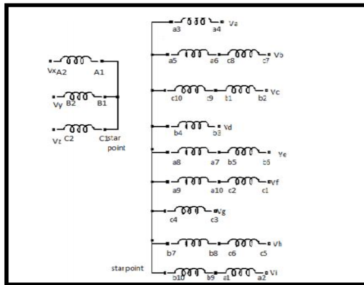
Fig. I. Proposed transformer winding connection (star-star).
