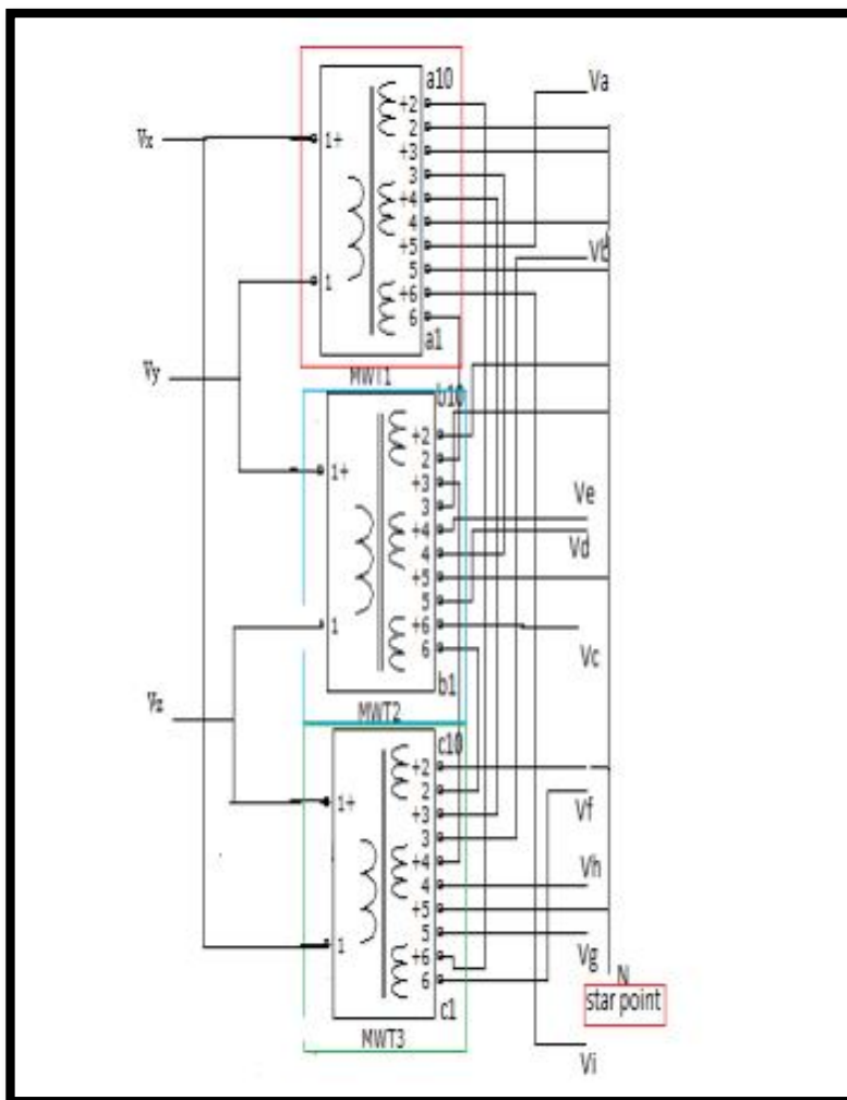
Fig V proposed winding arrangement (delta-star)
