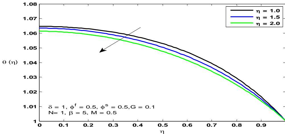
Figure 16. The temperature \theta(y) for different values of \eta
