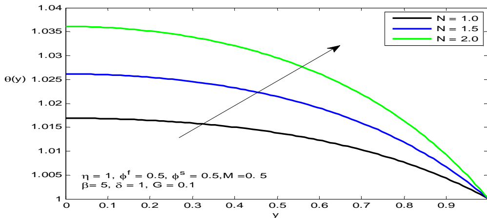
Figure 19. The temperature \theta(y) for different values of N
