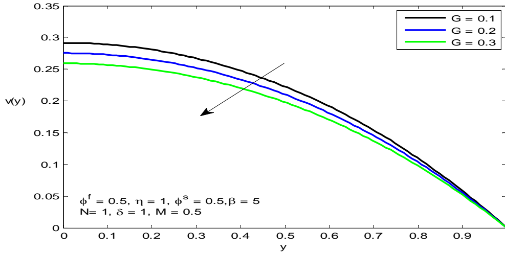
Figure 8. The velocity v(y) for different values of G
