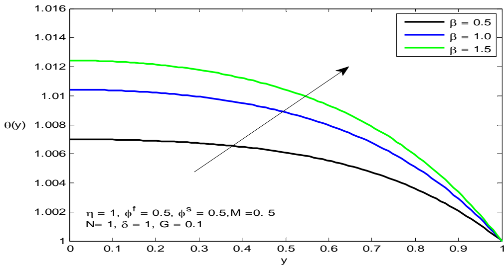
Figure 7. The temperature \theta(y) for different values of \beta
