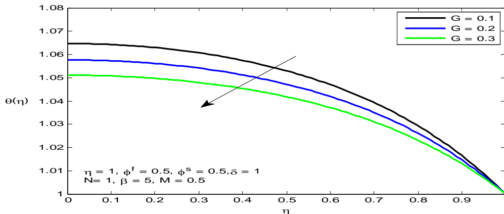
Figure 10. The temperature \theta(y) for different values of G
