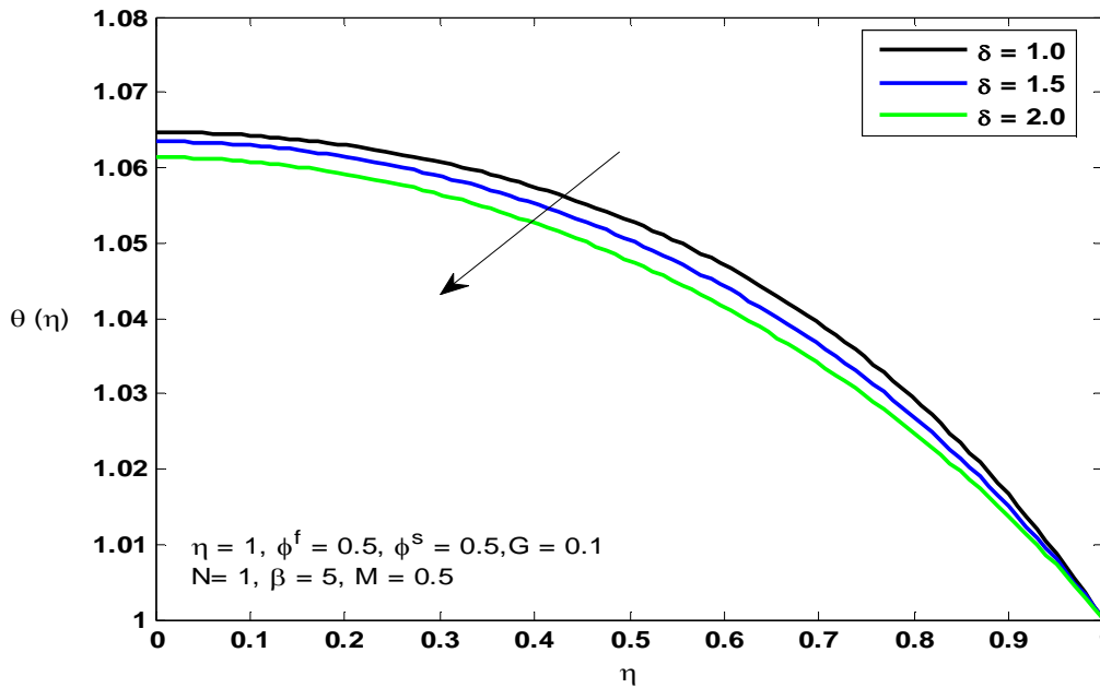
Figure 22. The temperature \theta(y) for different values of \delta
