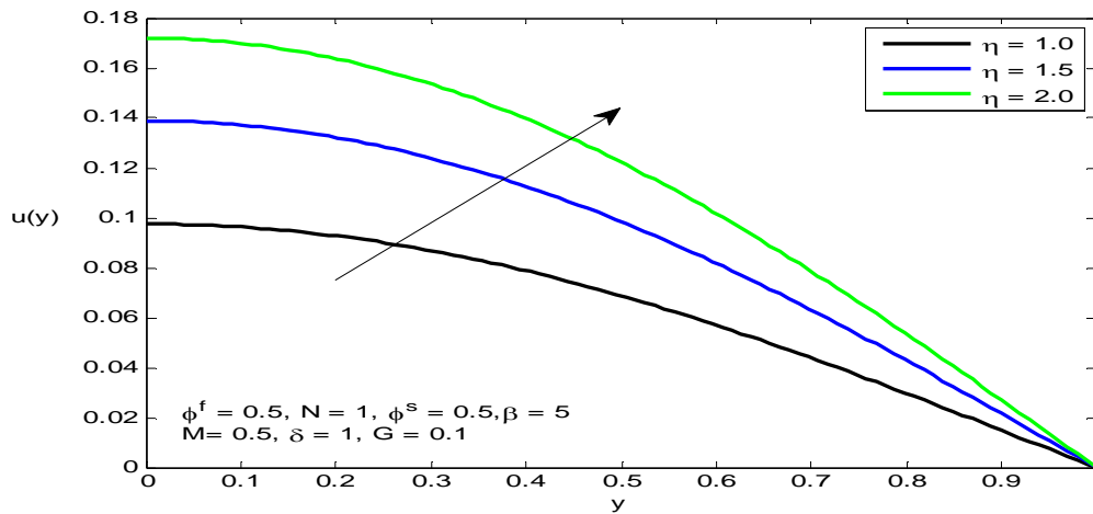
Figure 15. The displacement u(y) for different values of \eta
