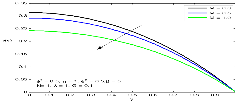
Figure 2. The velocity v(y) for different values of M
