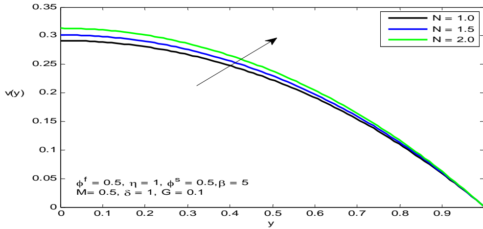
Figure 17. The velocity v(y) for different values of N
