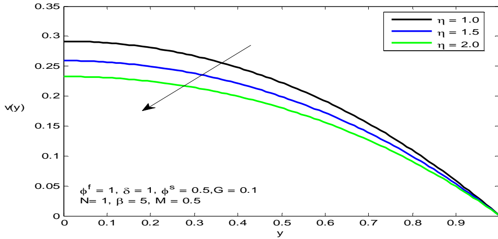
Figure 14. The velocity v(y) for different values of \eta
