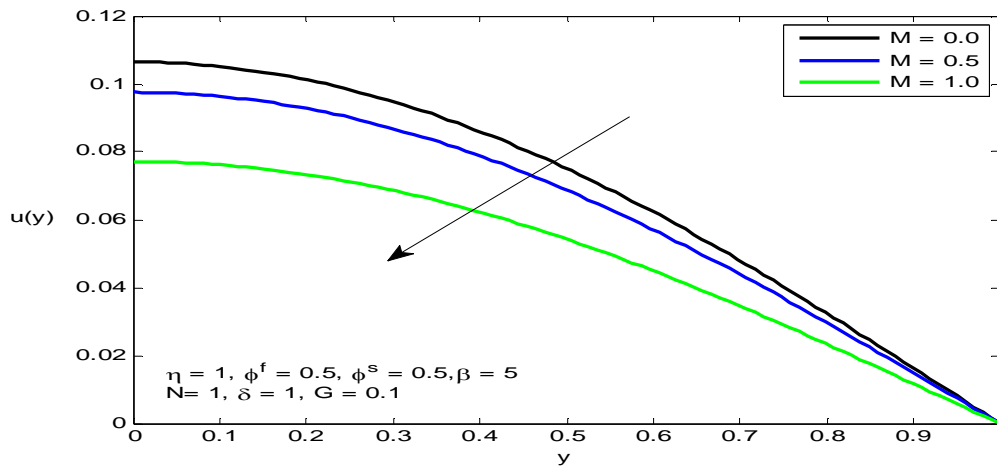
Figure 3. The displacement u(y) for different values of M
