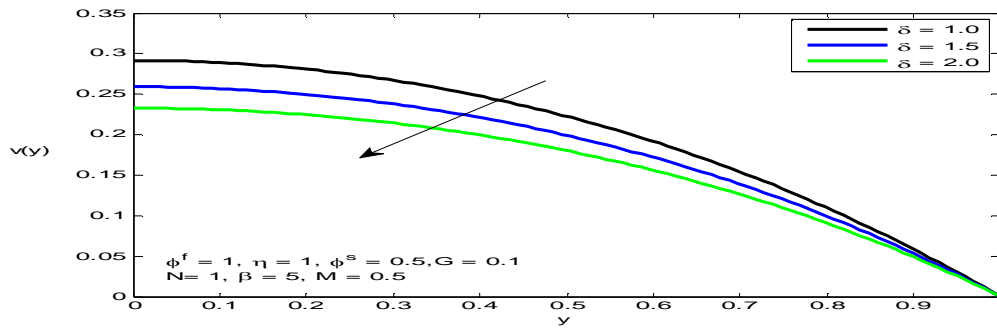
Figure 20. The velocity v(y) for different values of \delta
