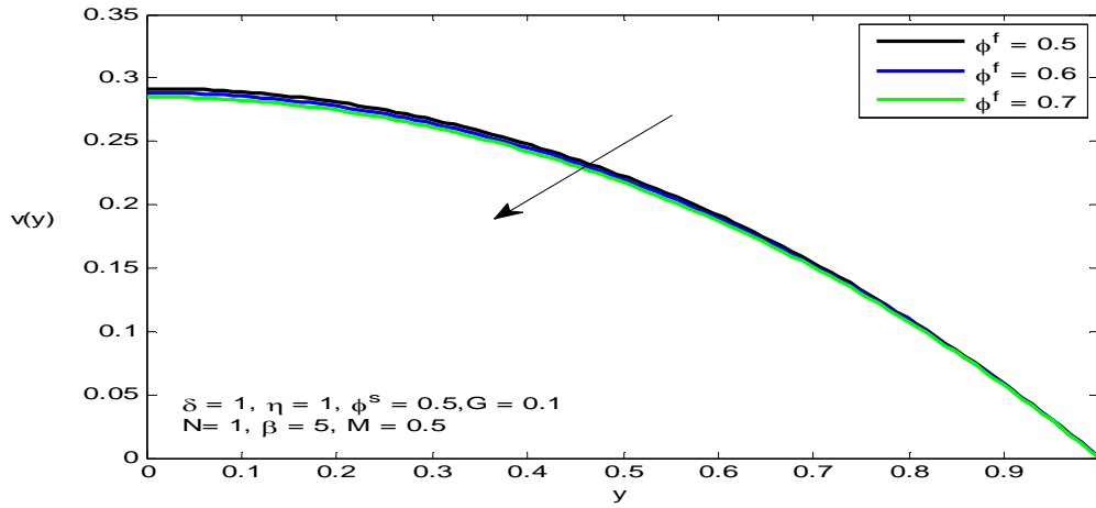
Figure 11. The velocity v(y) for different values of \phi^f
