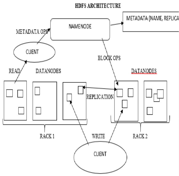
Figure 2.1 Hadoop Architecture
